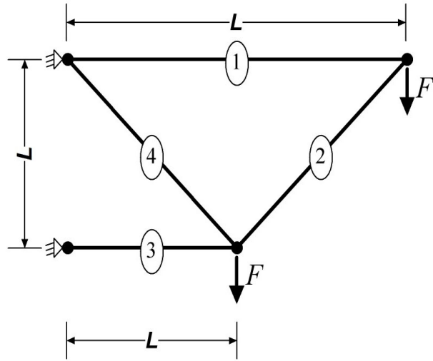
Fig. 13. 4-bar truss structure
