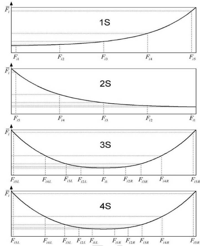
Fig. 1. The class-functions
