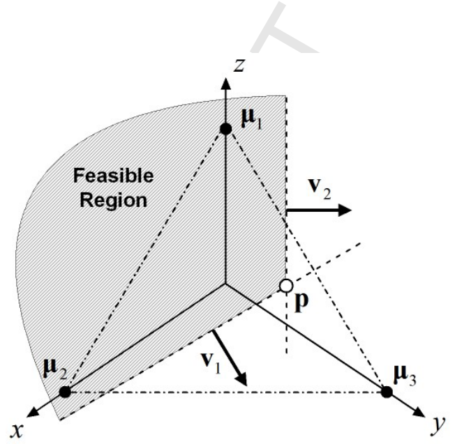
Fig. 11e. Feasible space in NC algorithm.
