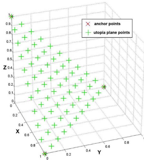
Fig. 11b. 3D test case. Utopia plane
