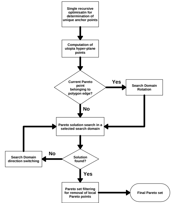
Fig. 7 Flowchart
