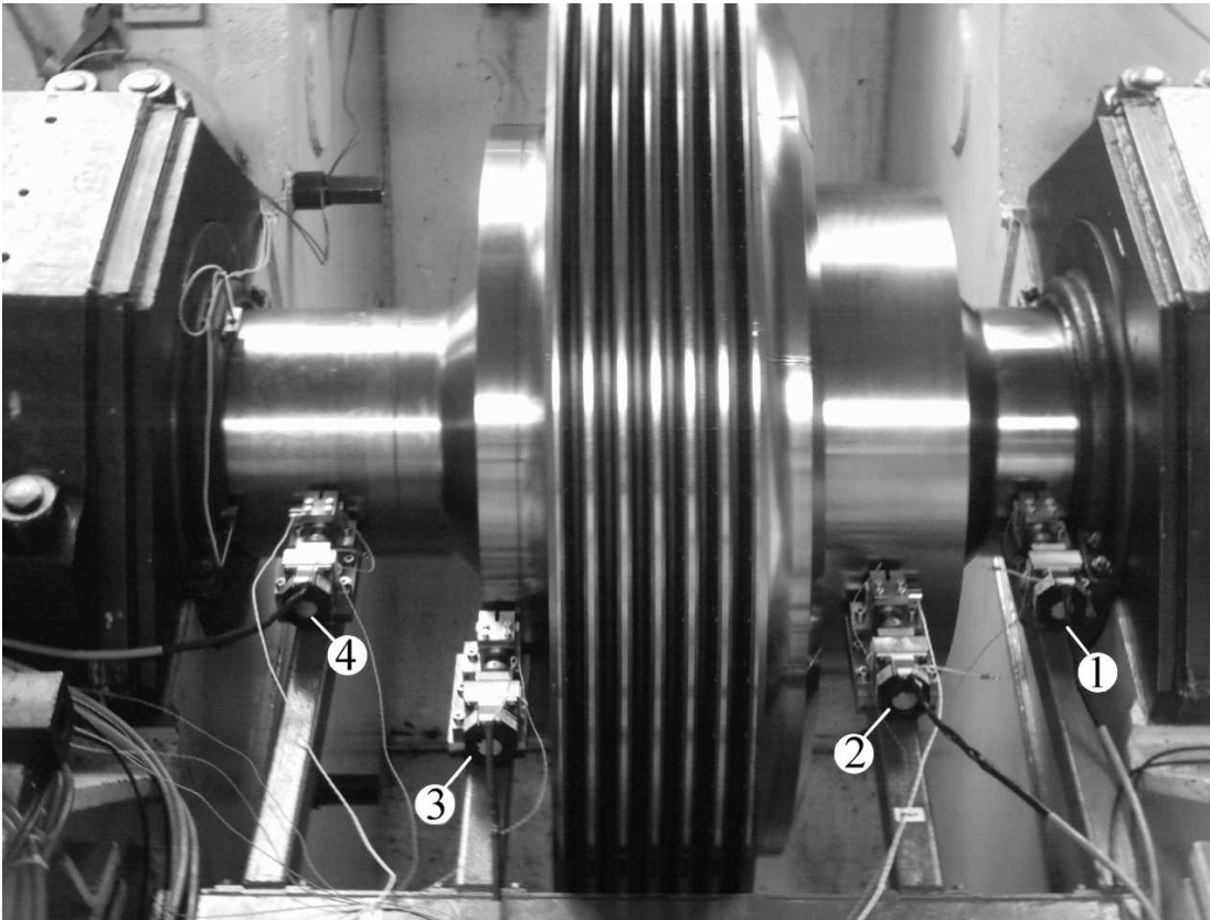
Figure 1: Test rig with the vacuum chamber lid removed. Drive-end is on the right.
