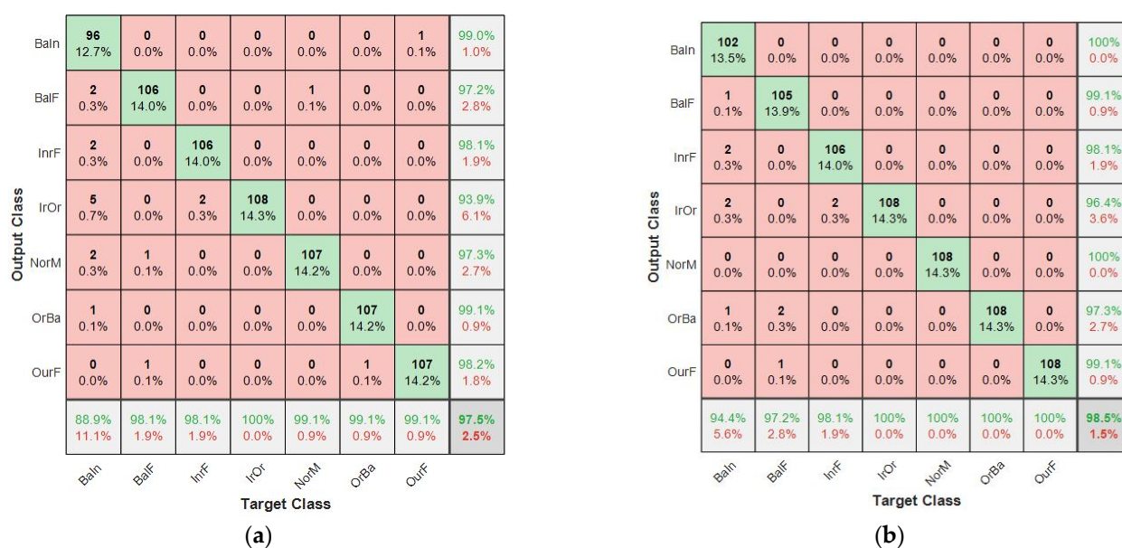
Figure 5. Confusion matrix for: (a) ECNN-DT; (b) proposed model (ECNN-SVM).
