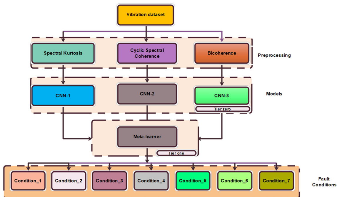
Figure 1. Proposed architecture for multiple faults of bearings.
