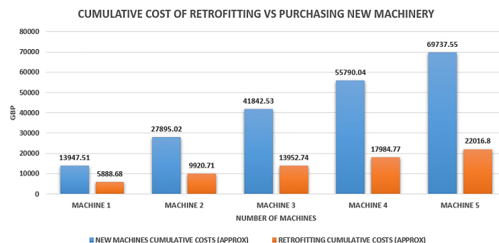
Fig. 4. – Comparison of the cumulative costs of retrofitting legacy lathe machines with I4 and AI-based RIS versus purchasing brand new I4-ready lathe machines followed by installation of RIS.
