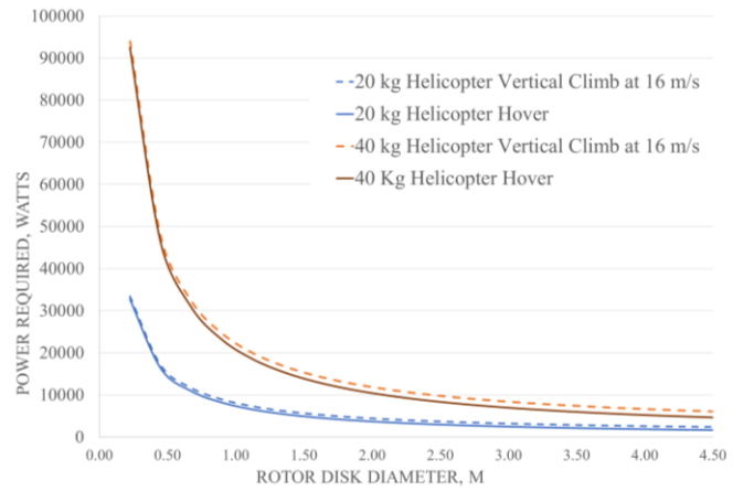
Fig. 3 Power Required vs Rotor Disk Diameter (Area) - 20 kg & 40 kg Martian Conventional Helicopter
