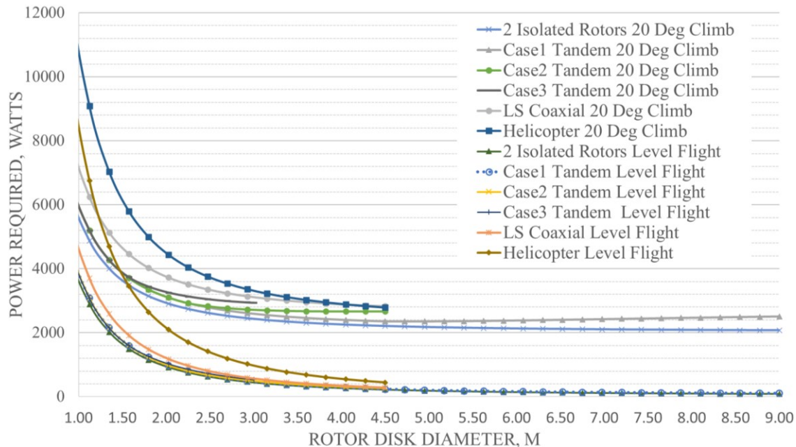
Fig. 8 Forward Flight Power Required (at 60.61 m/s) vs Rotor Disk Diameter (Area) – Comparison between various 20 kg rotorcraft configurations (2 Isolated Rotors, Tandem Cases, Coaxial, Helicopter)
