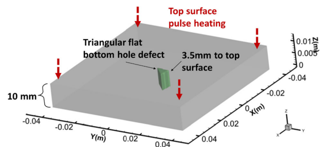
Fig. 4 Defective specimen model with a triangle shape flat bottom hole
