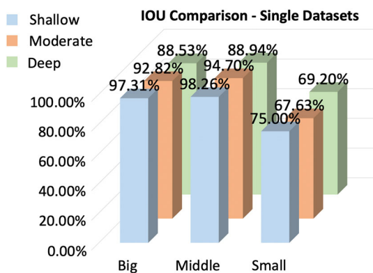
Fig. 8 Comparison of average intersection-over-union (IOU) of testing sets
