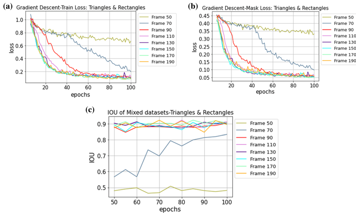
Fig. 12 Network performance comparison of thermal frames; a Overall train losses; b Mask losses; c IoU performance
