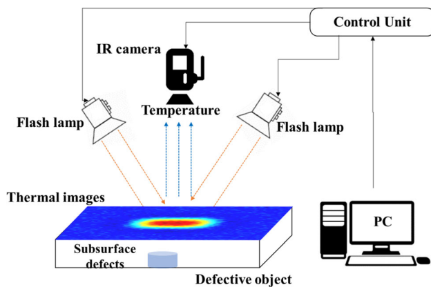
Fig. 1 The principle of pulsed thermography (PT)
