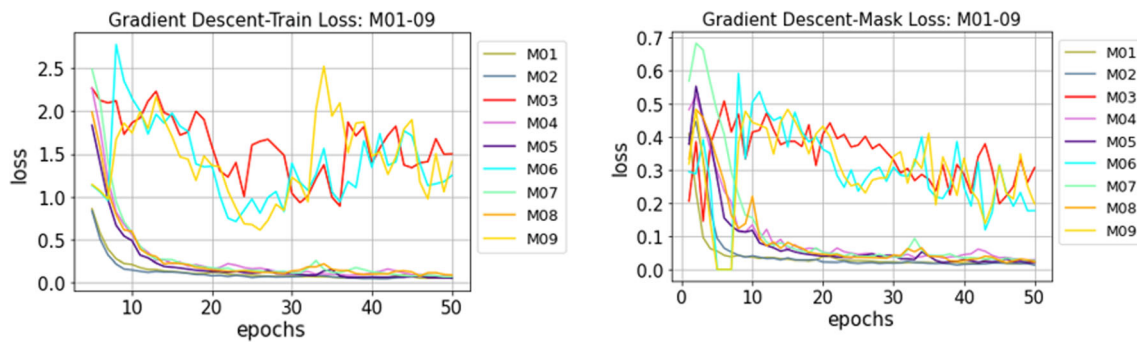
Fig. 9 Network loss in the training process; Left: Overall train losses of M01-09; Right: Mask losses of M01-09
