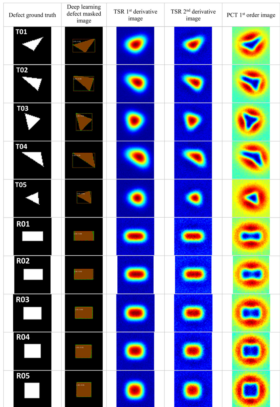
Fig. 11 Comparison of the network results with the TSR and PCT methods
