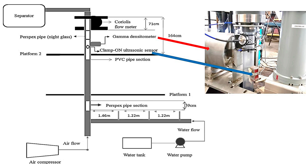
Figure 3. Experimental setup [25].
