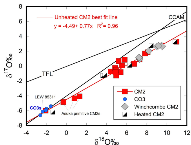
FIGURE 3. Winchcombe oxygen isotope analyses shown in relation to the oxygen isotope composition of CM2 and CO3 chondrites. All analyses were measured using the Open University laser fluorination line. The plot includes both published and previously unpublished analyses (see Table 2 for individual references). A best fit line through the CM2 data, excluding Winchcombe, intersects the CCAM line at the position where the CO3 falls plot. Some CM2 chondrites show evidence for heating subsequent to aqueous alteration (King et al., 2021). These heated CM2s were not included in the CM2 best fit line calculation. TFL, Terrestrial Fractionation Line; CCAM, Carbonaceous Chondrite Anhydrous Minerals line, Clayton and Mayeda (1999). (Color figure can be viewed at wileyonlinelibrary.com )
