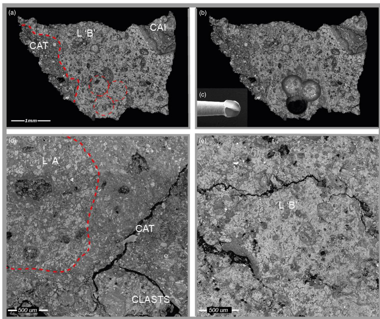
FIGURE 1. a) BSE image of polished block P30424 containing Lithology B (L'B') and cataclastic matrix (CAT) (proposed microsampling domains are outlined in red circles). The section also contains part of a calcium-aluminum-rich inclusion (CAI). b) Polished block P30424 showing micromilled excavations. The targeted resolution of the micromill permits sampling of material that is dominated by aqueous alteration products. The lowermost excavation appears black at the base. This indicated that the micromill had penetrated epoxy resin, and therefore, only the powders from the top two holes were used. c) A ball-point tungsten carbide tip used in this work. d) BSE image of polished block BM.2022, M1-123, where the sampled regions of Lithology A (L'A') and the cataclastic matrix (CAT) are visible. e) BSE image of polished block BM.2022, M1-117, which contains Lithology B (L'B') only. (Color figure can be viewed at wileyonlinelibrary.com )
