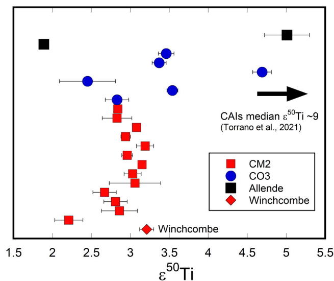
FIGURE 13. \varepsilon^{50}\text{Ti} comparison between CM2 chondrites, CO3 chondrites, and Allende (CV3). See text for discussion. Data compiled from Trinquier et al. (2009), Zhang et al. (2011, 2012), Torrano et al. (2021), this study. (Color figure can be viewed at wileyonlinelibrary.com )
