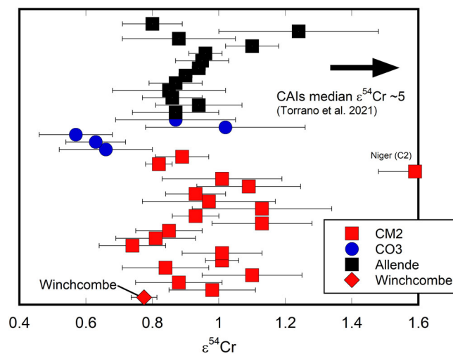
FIGURE 14. \varepsilon^{54}\text{Cr} comparison between CM2 chondrites, CO3 chondrites, and Allende (CV3). See text for further discussion. Data compiled from Shukolyukov and Lugmair (2006a, 2006b), Trinquier et al. (2007), Trinquier, Birck, & Allègre (2008), Trinquier, Birck, & Allègre, et al. (2008), Qin, Alexander, et al. (2010), Qin, Rumble, et al. (2010), Jenniskens et al. (2012), Gopel et al. (2015), Van Kooten et al. (2020), Zhu et al. (2020), Zhu, Moynier, Schiller, Becker, et al. (2021), Williams et al. (2020), Torrano et al. (2021). (Color figure can be viewed at wileyonlinelibrary.com )
