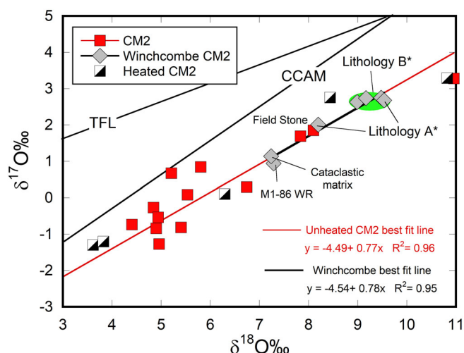
FIGURE 4. Oxygen isotope plot showing the relationship between the various Winchcombe lithologies. Lithology B (highlighted in green) was measured in three samples: M1-85 (bulk); microdrilled fraction from polished block M1-177 and microdrilled fraction from polished block P30424. Lithology A was sampled by a microdrilled fraction from polished block M1-123 and is also the main constituent of the Field Stone (Suttle et al., 2022). Cataclastic matrix was sampled by a micromilled fraction from polished block M1-123. The bulk sample from stone M1-86 appears to have sampled a significant proportion of cataclastic matrix. The best fit line through the Winchcombe analyses is almost identical to the CM2 unheated best fit line (Figure 3). *Lithological designation based on the criteria of Suttle et al. (2022). (Color figure can be viewed at wileyonlinelibrary.com )
