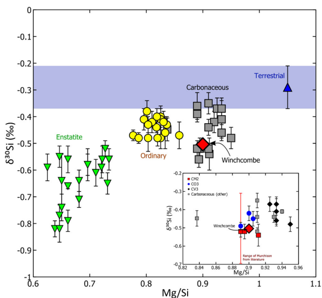
FIGURE 12. Silicon isotope composition of Winchcombe CM2 meteorite versus its Mg/Si (by weight) ratio (red diamond). Also shown are literature data for other chondritic meteorites (Armstrong et al., 2011; Chakrabarti & Jacobsen, 2010; Fitoussi et al., 2009; Savage & Moynier, 2013; Zambardi et al., 2013) and an estimate for the composition of the bulk silicate Earth (Savage et al., 2014). Inset: expanded view of the carbonaceous chondrite data, with the literature CM, CO, and CV analyses highlighted. The Winchcombe Si isotope composition matches well with previous measurements of other CM2 material; CO3 meteorites appear to be slightly isotopically heavier than CM2; see text for further details. The Mg/Si ratios of the meteorites were calculated using data held on Metbase. The Mg/Si ratio of Winchcombe, 0.9, is based on analysis by A. J. King (personal communication). (Color figure can be viewed at wileyonlinelibrary.com )
