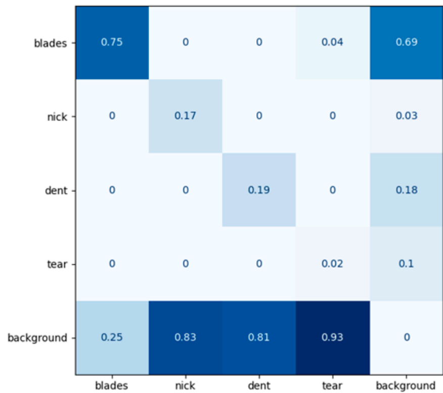
Figure 7. Normalized confusion matrix of Model2_100.
