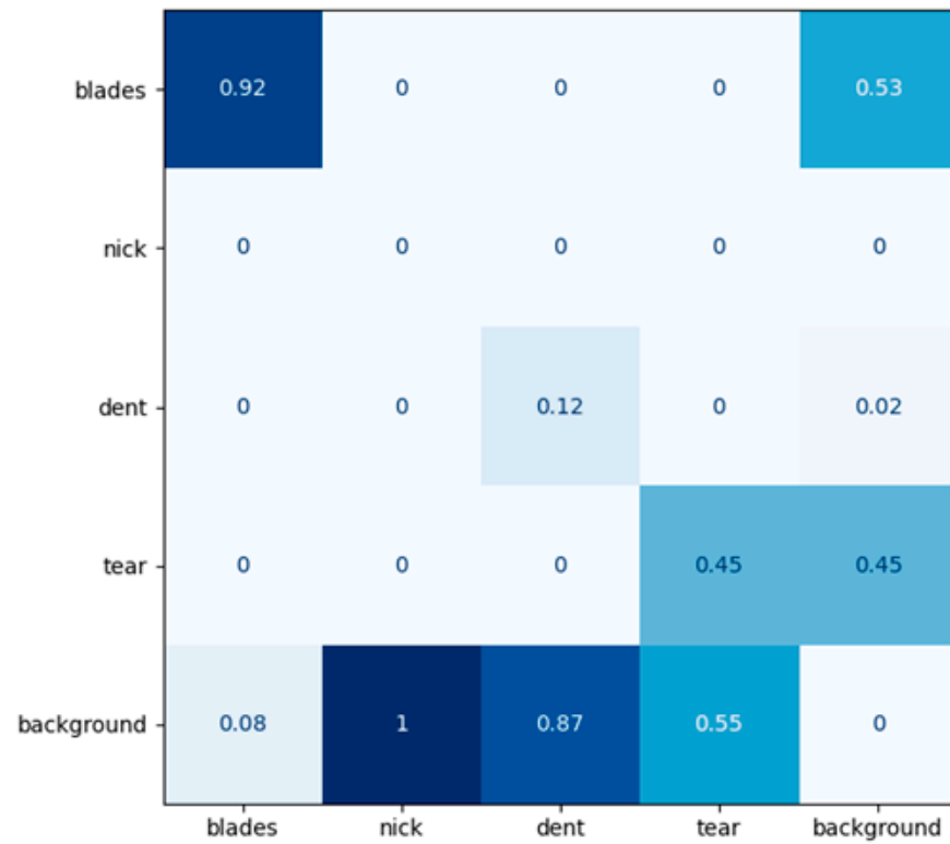
Figure 9. Normalized confusion matrix of Model3_50v1.
