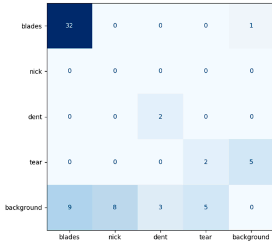
Figure 6. Confusion matrix of Model1_100.
