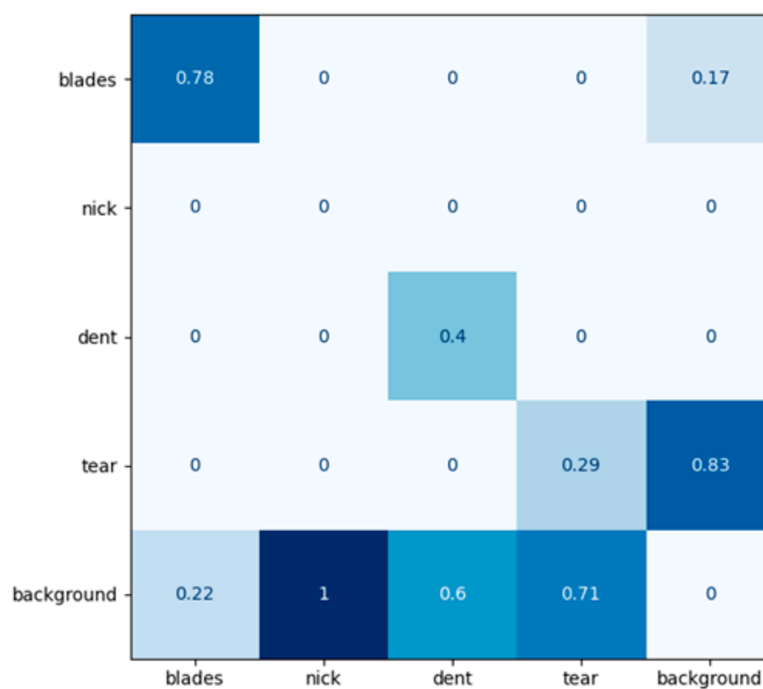
Figure 5. Normalized confusion matrix of Model1_100.
