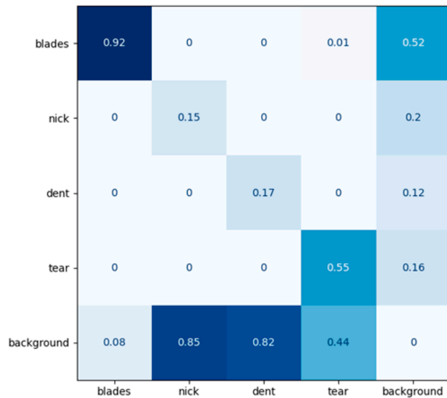
Figure 12. Normalized confusion matrix of Model3_100.
