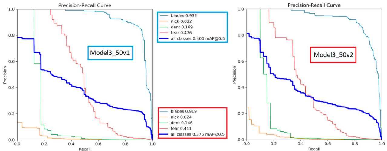
Figure 11. Precision/recall curves for Model3_50v1 and Model3_50v2.
