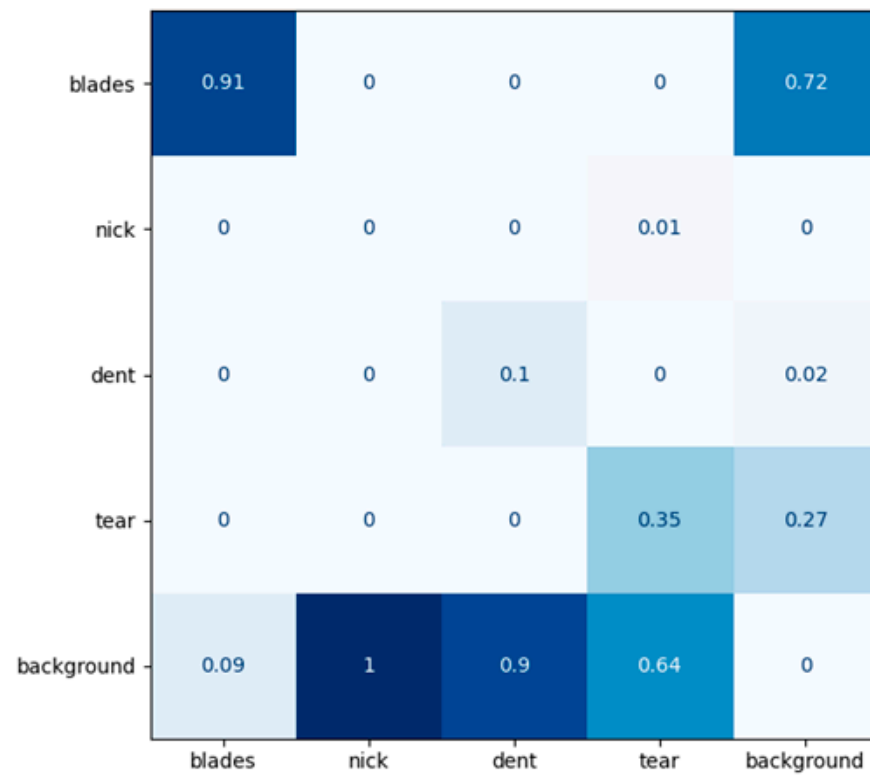
Figure 10. Normalized confusion matrix of Model3_50v2.
