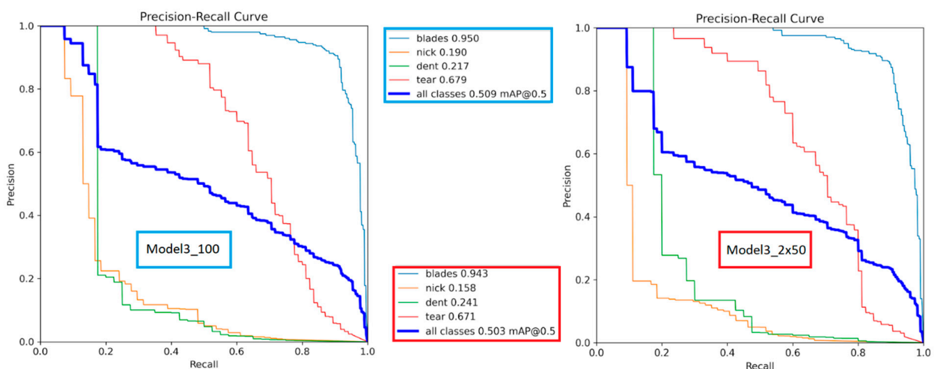
Figure 14. Precision/recall curves for Model3_100 and Model3_2x50.
