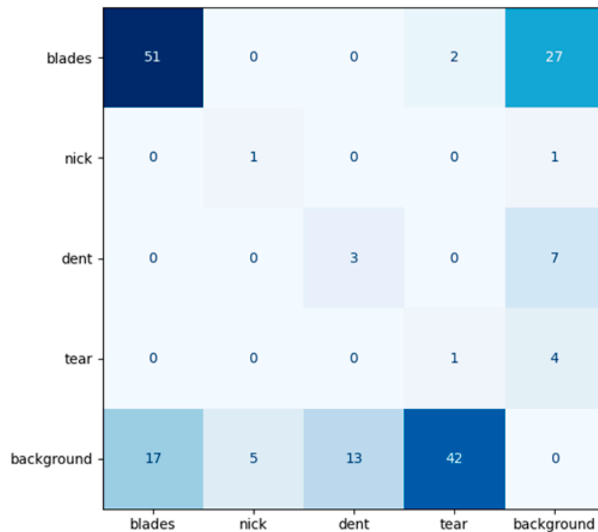
Figure 8. Confusion matrix of Model2_100.
