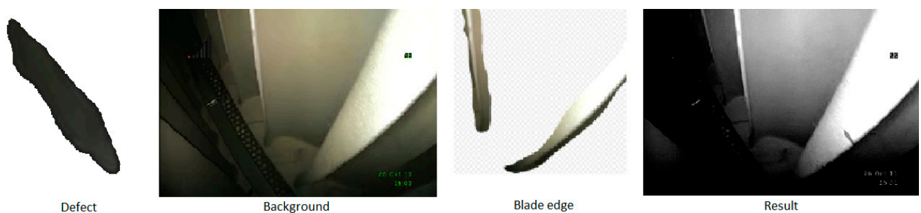
Figure 19. A synthetic image with a defect on the blade edge.
