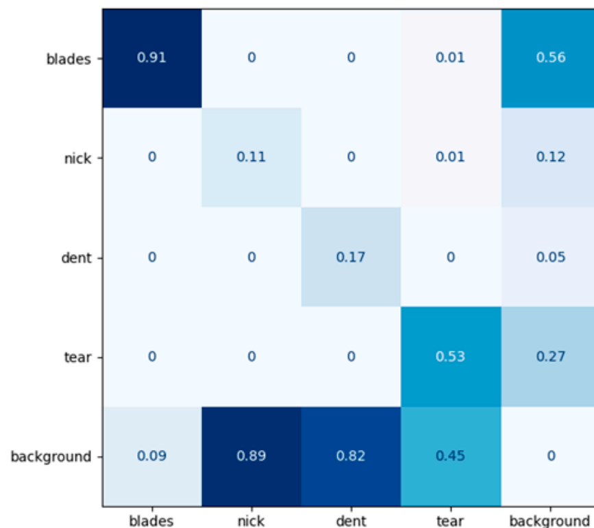
Figure 13. Normalized confusion matrix of Model3_2x50.
