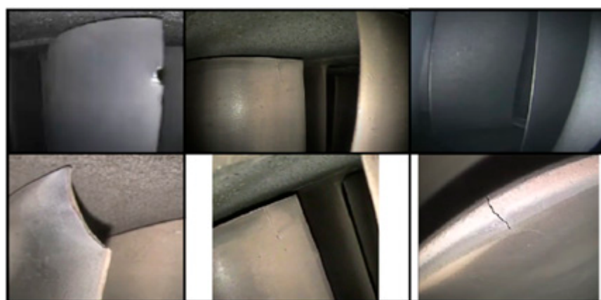
Figure 4. Example images from Dataset 1 with wide view ( top ) and Dataset 2 with zoom-in view ( bottom ).
