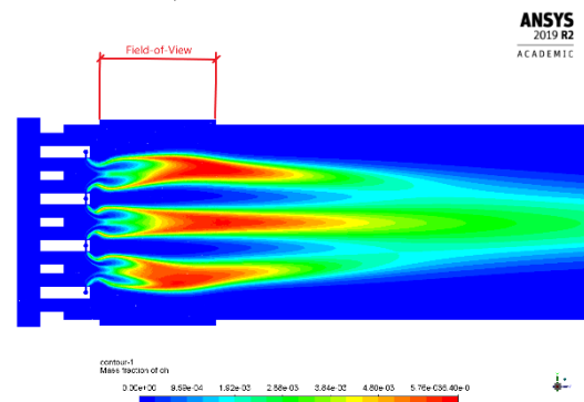
Figure 9 - Flame length against the size of field-of-view. Simulation at atmospheric pressure
