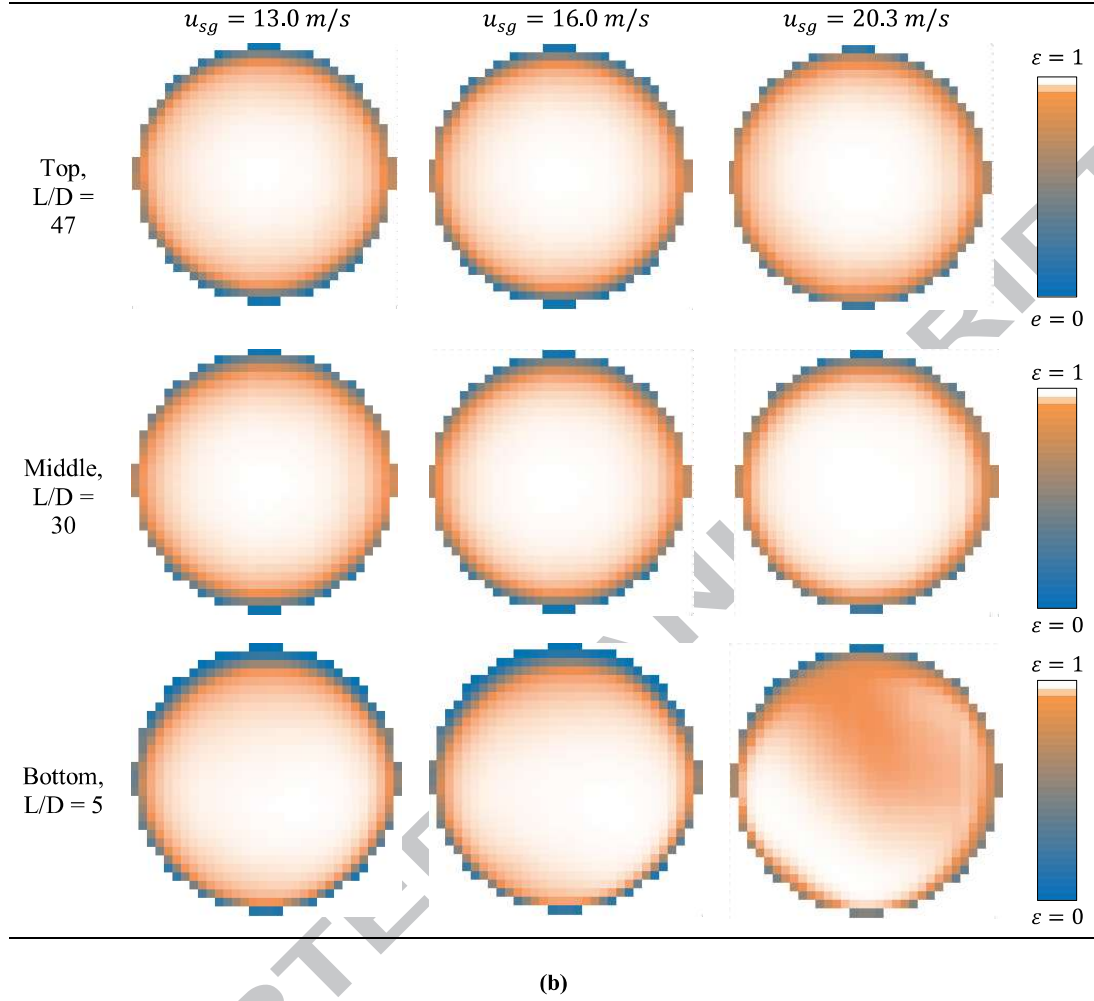
Figure 6: Sample reconstructed time-averaged WMS images for upward flow at (a) u_{sl} = 0.30 \text{ m/s} (top), and (b) u_{sl} = 1.0 \text{ m/s} (bottom). Taken at L/D = 5, 30 , and 47 from BEND2. Blue indicates water at low void fraction ( \epsilon ) values, white indicates air at \epsilon \rightarrow 1 , and orange indicates entrained liquid droplets at intermediate \epsilon values.
