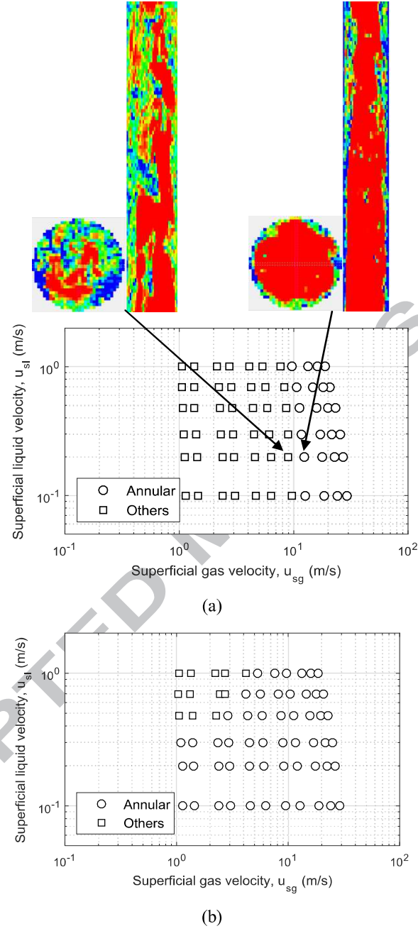
Figure 9: Flow regime maps obtained for (a) upward (see Aliyu et al. [54]) and (b) downward flow. . Snapshots of videos produced using stacked WMS images of flow at u_{sl} = 0.2 m/s were used to differentiate between churn and annular flows at u_{sl} = 9.7 , and 14.1 m/s respectively
