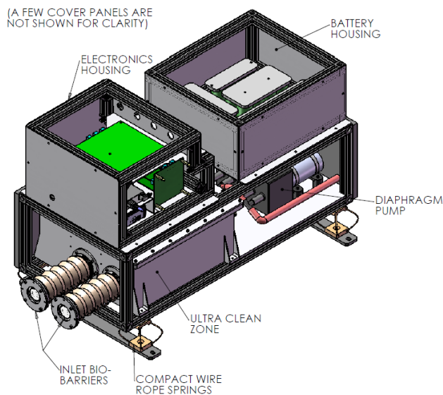
Fig 3: CASS•E assembly (left) & CASS•E in 'S-Egon' 1 gondola with communications 'E-Link' 1 system (right).
