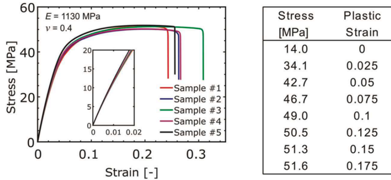
Fig. 10. Elastic and plastic material properties for Nylon PA2200.
