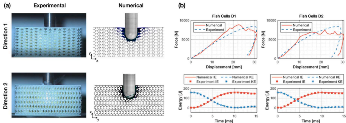
Fig. 12. (a) Comparison of results from the experimental analysis and numerical models for Fish Cells lattice structure deformation in D1 and D2. (b) Force-displacement curves, internal and kinetic energy vs time curves obtained from the experimental and numerical analyses.
