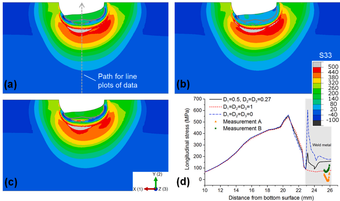
Fig. 7. Longitudinal residual stresses in the 3-pass GTA welded plate: (a) prediction when D_1 = 0.50 , D_2 = D_3 = 0.27 ; (b) prediction when D_1 = D_2 = D_3 = 1 ; (c) prediction when D_1 = D_2 = D_3 = 0 ; (d) through-thickness distribution along weld centreline. Note that D_n indicates the dilution for pass n . Solid and dashed grey lines in (a)–(c) indicate the predicted current and accumulated fusion boundaries, respectively.
