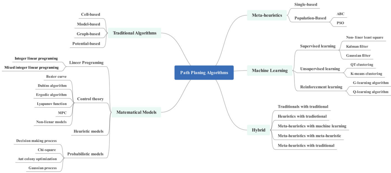
Figure 8. Classification of the path planning algorithms for UAVs (adapted from Refs [51, 56]).
