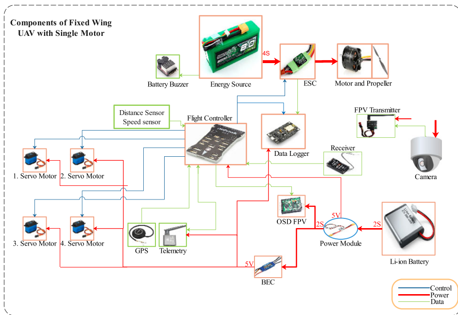
Figure 7. Electronic equipment of a small fixed-wing UAV with a single motor.
