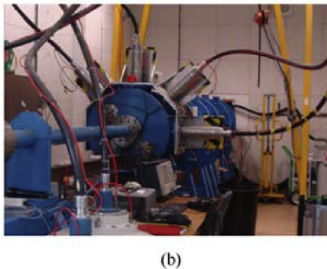
Fig. 4. Reverse ballistic experimental configuration: (a) schematic illustration; (b) external picture of target chamber with flash X-ray heads (silver tubes) arrayed around target position.
