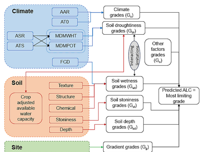
Fig. 1. Calculation of ALC limiting criteria from climate, soil, and site data. AAR: Average annual rainfall; ASR: Average summer rainfall (April to September); AT0: Accumulated temperature (January to June); ATS: Accumulated temperature (April to September); FCD: Field capacity days; MDMWHT/MDMPOT: Moisture deficit for wheat/potato. Please see supplementary information S1 for more information on these parameters.
