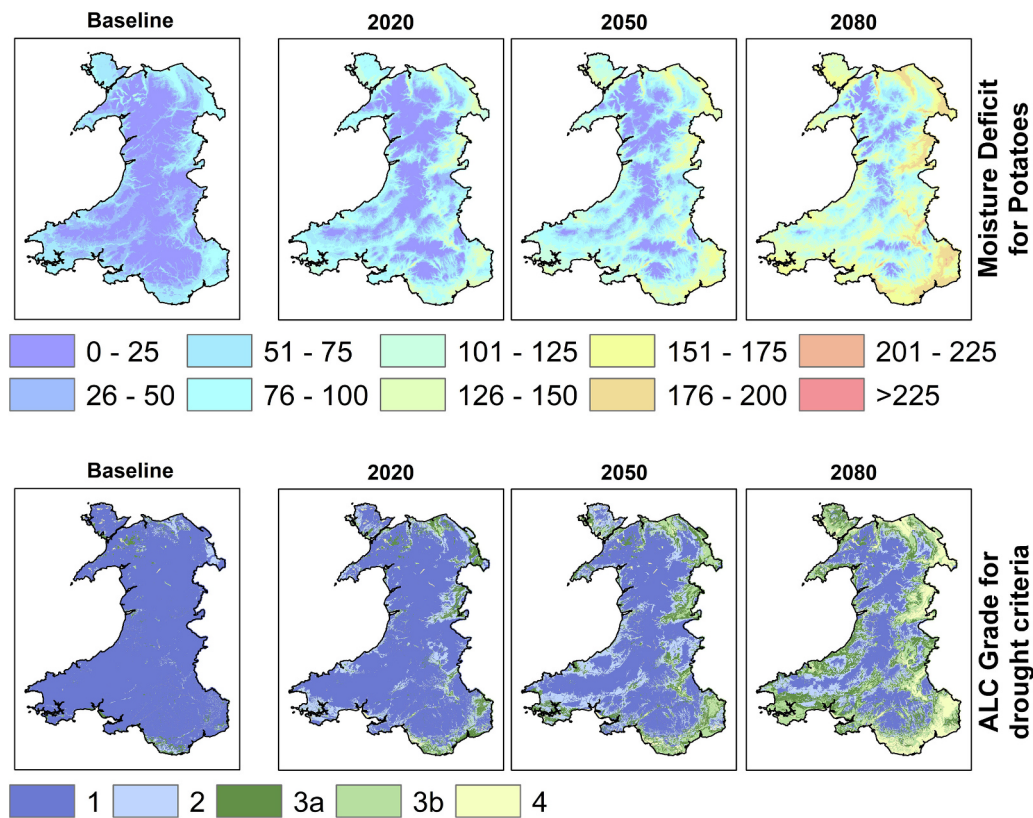
Fig. 3. Moisture deficit (mm) for potatoes (above) and ALC grade for drought criteria (below) for baseline climate (1961–1990), 2020, 2050 and 2080 for RCP 4.5 emission scenario.
