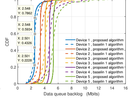
Fig. 4. CDF of data queue backlog.
