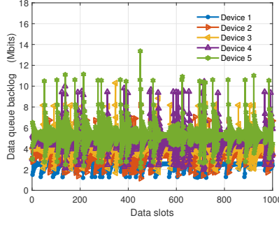
Fig. 3. Data queue backlog of the baseline 1 algorithm.
