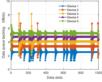
Fig. 2. Data queue backlog of the proposed algorithm.
