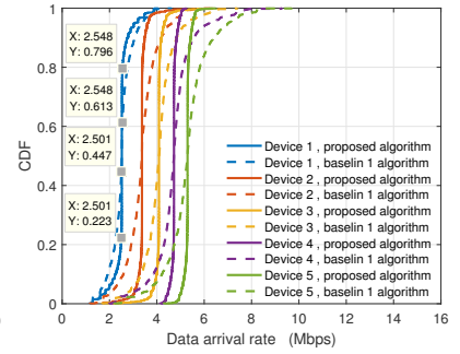
Fig. 7. CDF of data arrival rate.
