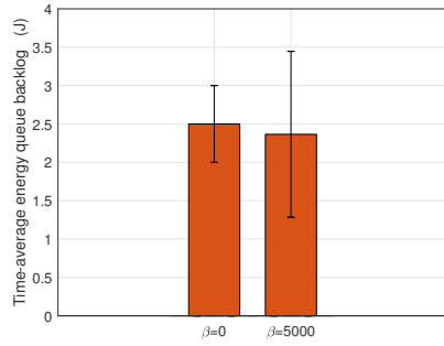
Fig. 17. Time-average energy queue backlog with standard deviation. Fig. 18. Convergence of primal variables. Fig. 19. Convergence of dual variables.
