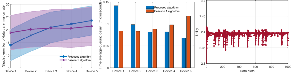
Fig. 8. Shaded error bar of transmission rate. Fig. 9. Time-average queueing delay. Fig. 10. Network utility of the proposed algorithm.
