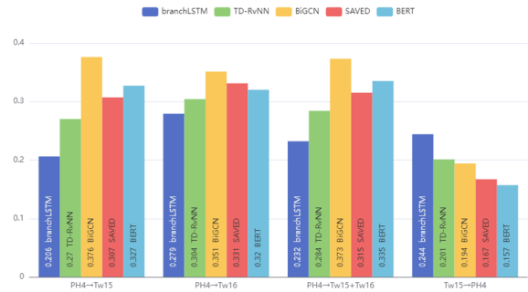
Figure 6: Cross-dataset evaluation of models train and test on different datasets, such as training on PHEME, testing on Twitter15/Twitter16 and vice versa.
