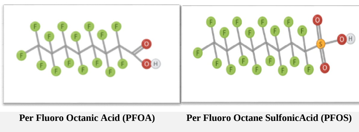
Fig.1 The Chemical structure of two important compounds of PFAS class that are PFOA and PFOS, showing their strong Carbon-Fluorine backbone
