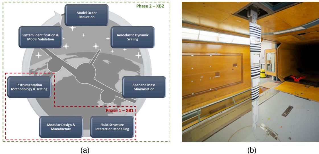
Figure 1 – BearDS work flow (retrieved from [1]) and XB-2 in the 8'x6' Cranfield University wind tunnel (retrieved from [4]).
