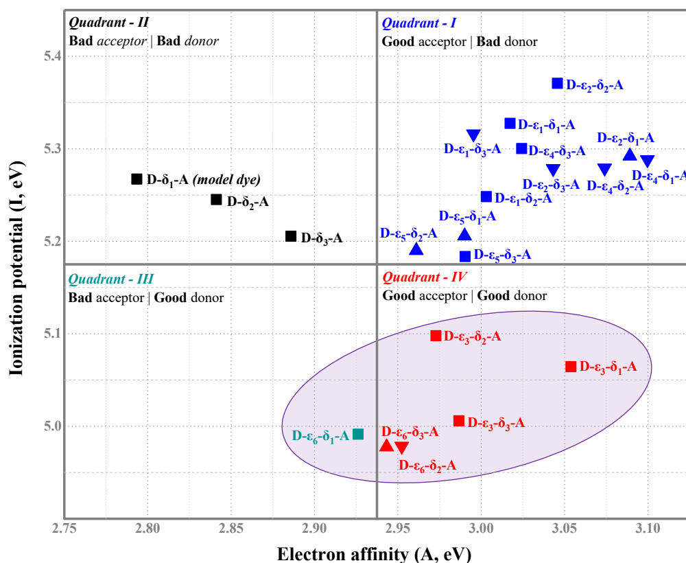
Figure 4. Full-electron-donor-acceptor map of the investigated photosensitizers (I and A values predicted via delta -SCF method) [M06-2X//6-31G(d,p) solvent model: CPCM, \epsilon_{\text{ethanol}} = 24.55 ].
