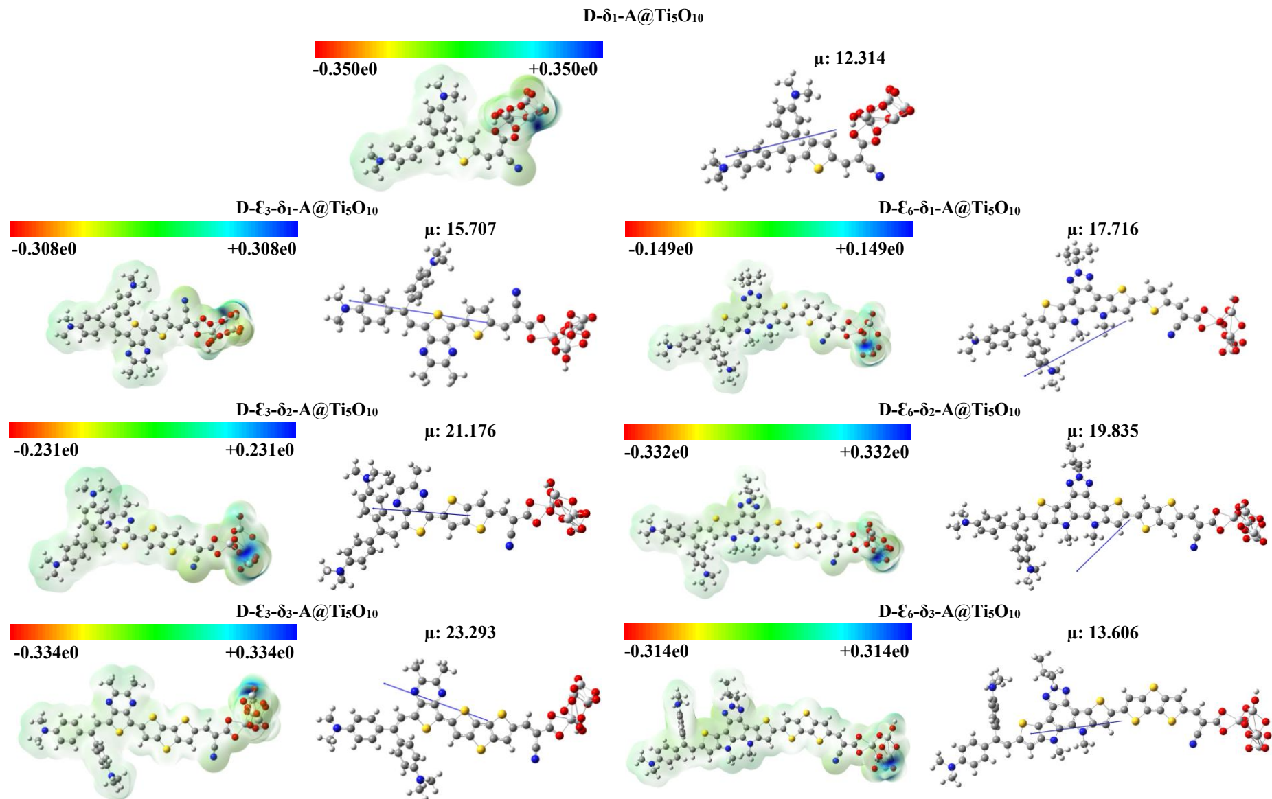
Figure 9. ESP maps and total dipole moment vectors of the investigated dye@Ti 5 O 10 clusters [M06-2X//6-31G(d,p) solvent model: CPCM, \epsilon_{\text{ethanol}}=24.55 ].
