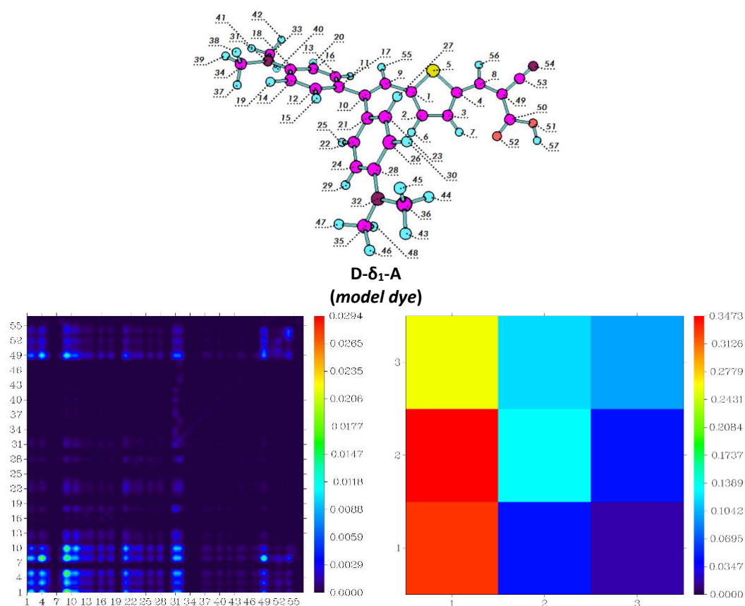
Figure 7. Atom- and fragment-based transition density and color correlation matrix (where the y-axis is the originating, and the x-axis is the receiving fragment for the excited electron) of the model dye [M06-2x/6-31G(d,p) solvent model: CPCM, \epsilon_{\text{ethanol}} = 24.55 ].
