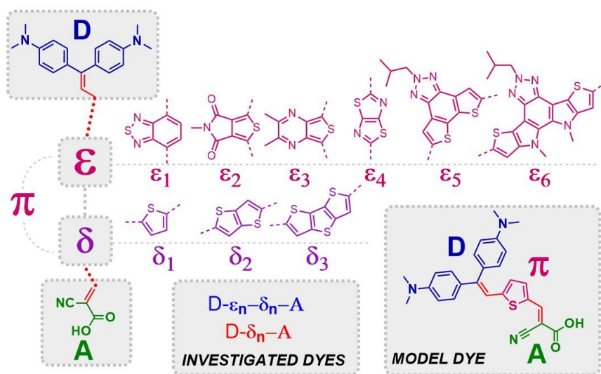
Figure 1. Structure of the model dye and the chemical scheme of the investigated D- \pi -A photosensitizers.
