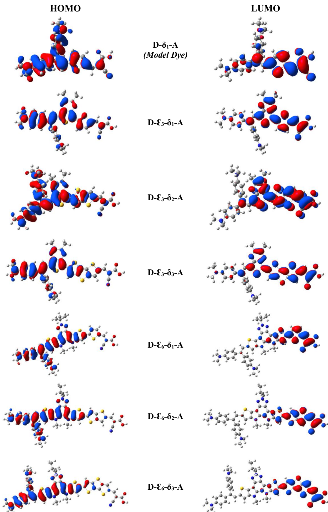
Figure 3. HOMO and LUMO contour plots of the investigated D-E 3 - \delta_n -A and D-E 6 - \delta_n -A systems. The threshold of contours is \pm 0.02 au [M06-2X/6-31G(d,p) solvent model: CPCM, \epsilon_{\text{ethanol}} = 24.55 ].
