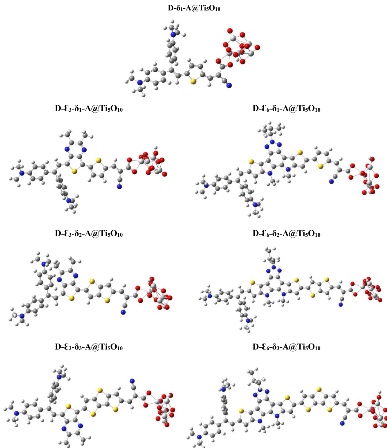
Figure 8. Geometry optimized molecular structures of the investigated dye@Ti 5 O 10 clusters [M06-2X//6-31G(d,p) solvent model: CPCM, \epsilon_{\text{ethanol}}=24.55 ].
