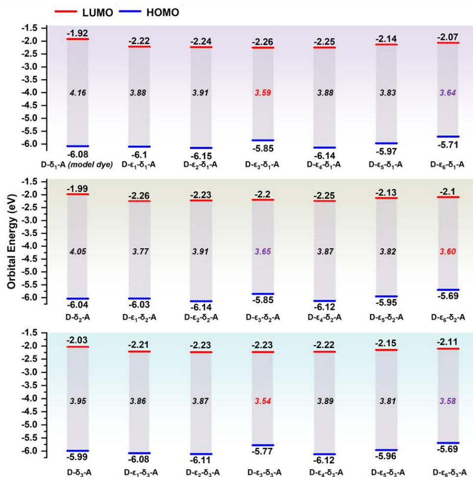
Figure 2. Computed HOMO, LUMO, and bandgap energies of the D- \pi -A photosensitizers [M06-2X/6-31G(d,p) solvent model: CPCM, E_{\text{ethanol}} = 24.55 ].
