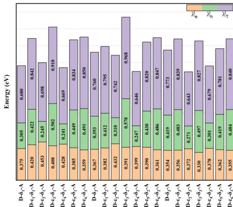
Figure 5. Calculated reorganization energies ( \lambda_e , \lambda_h , \lambda_T ) [M06-2X//6-31G(d,p)].
