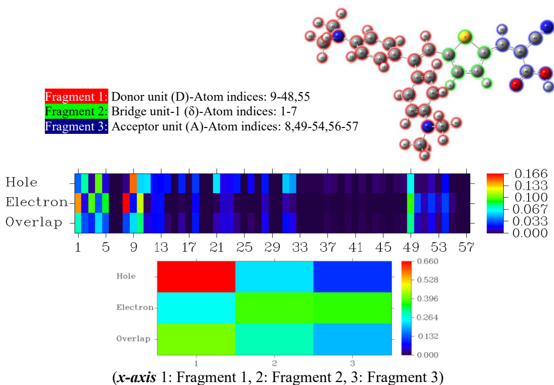
Figure 6. Atom- and fragment-based electron-hole distribution of model dye (D- \delta_1 -A)
