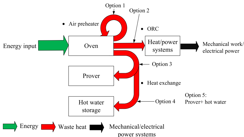
Fig. 3. Selected waste heat recovery options for commercial bakeries.
