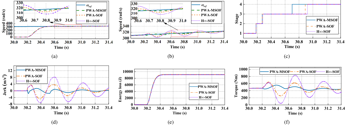
Fig. 6. Comparison of proposed PWA-MSOF, PWA-SOF and H_\infty -SOF. a Comparison of clutch driven disc speed. b Comparison between clutch driving disc speed and reference speed. c Comparison of MTP stage. d Vehicle jerk. e Slipping energy loss. f Torque transmitted to the wheels.
