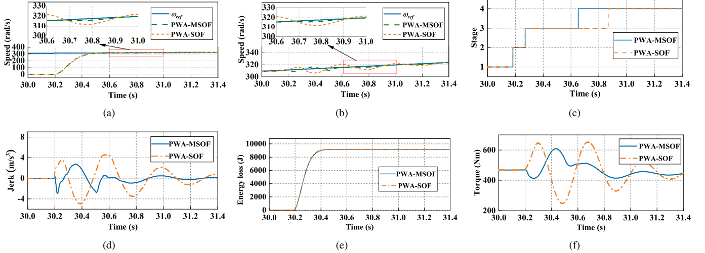
Fig. 10. Comparison of proposed PWA-MSOF and PWA-SOF in HiL test. a Comparison of clutch driven disc speed. b Comparison between clutch driving disc speed and reference speed. c Comparison of MTP stage. d Vehicle jerk. e Slipping energy loss. f Torque transmitted to the wheels.
