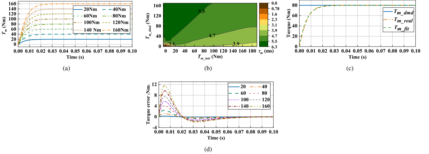
Fig. 4. Dynamic characteristics of PMSM. (a)Response characteristics of PMSM. (b)Mechanical hysteresis of PMSM. (c)Torque comparison of PMSM. (d)Torque error comparison of PMSM.
