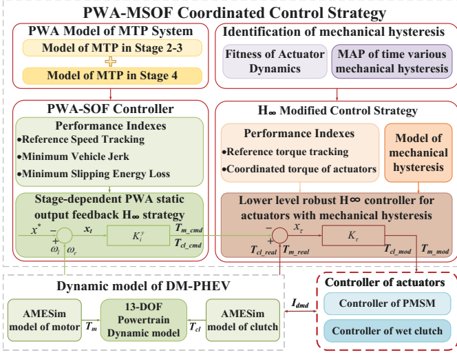
Fig. 5. Coordinated control architecture.
