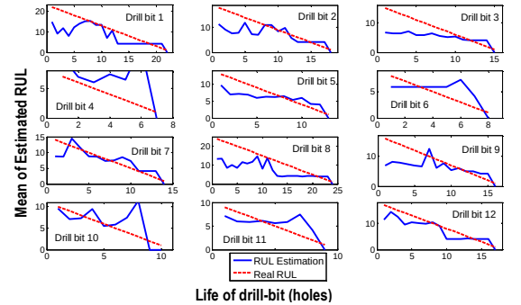
(b) Plots of estimated RUL along with true RUL for all 12 drill-bits
