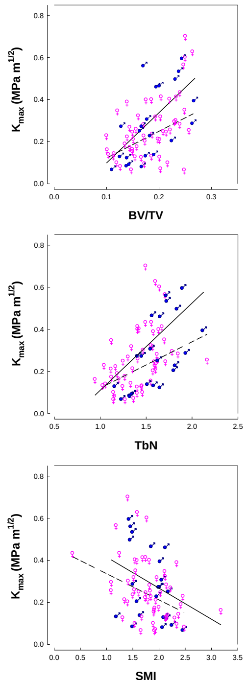
Figure 1: Critical stress intensity ( K_C ) as a function of various microarchitectural properties: (A) BV/TV; (B) TbN; (C) SMI. Male (♂) Female (♀).
