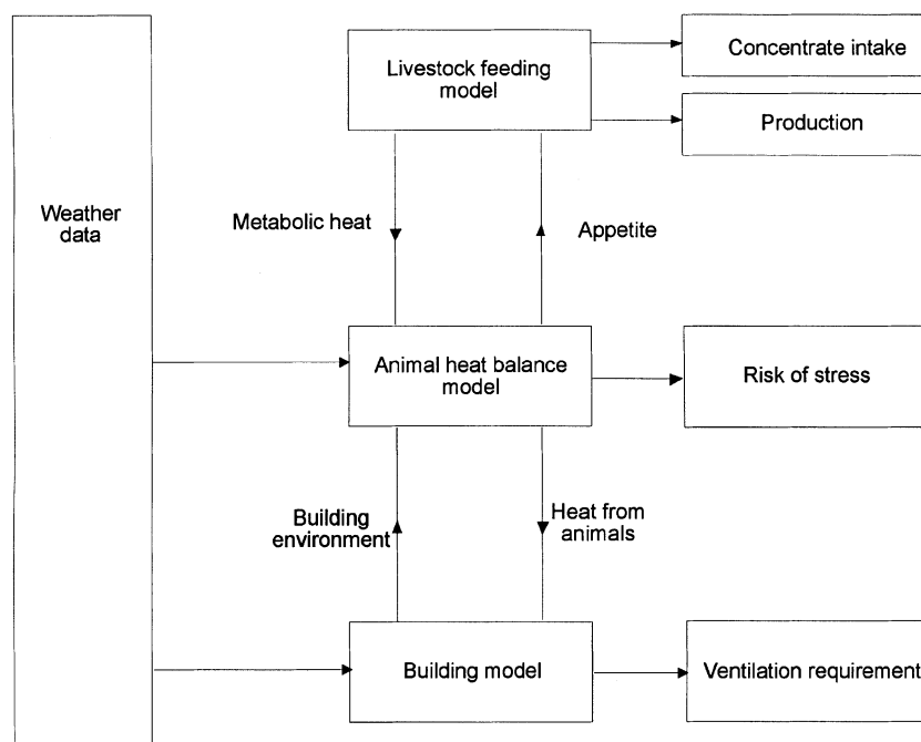
Fig. 1 Schematic of the intensive livestock integrated model
