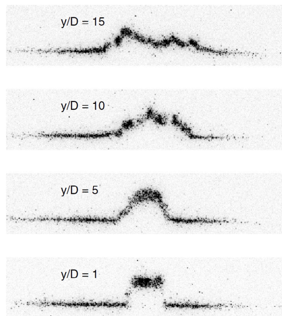
Fig. 13. Single-shot images of displaced FLEET lines at different downstream locations corresponding to heights above the jet exit of 1, 5, 10, and 15 mm. Fluorescence is collected 2 \mu s after the tagging laser, and the camera gate width is 1 \mu s. The unperturbed flow position is indicated by the fluorescent lines outside of the free jet.
