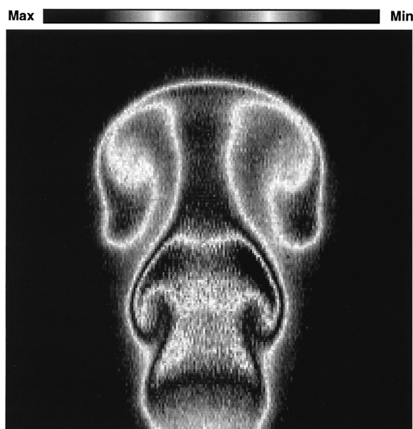
Fig. 12. Example CO 2 LIF visualisation of a 6-mm-diameter forced CO 2 jet at room-temperature mixing with ambient air. The fluorescence signal is excited with a 8 mJ pulse at 2.0 \mu m and an InSb camera collects fluorescence at 4.3 \mu m.
