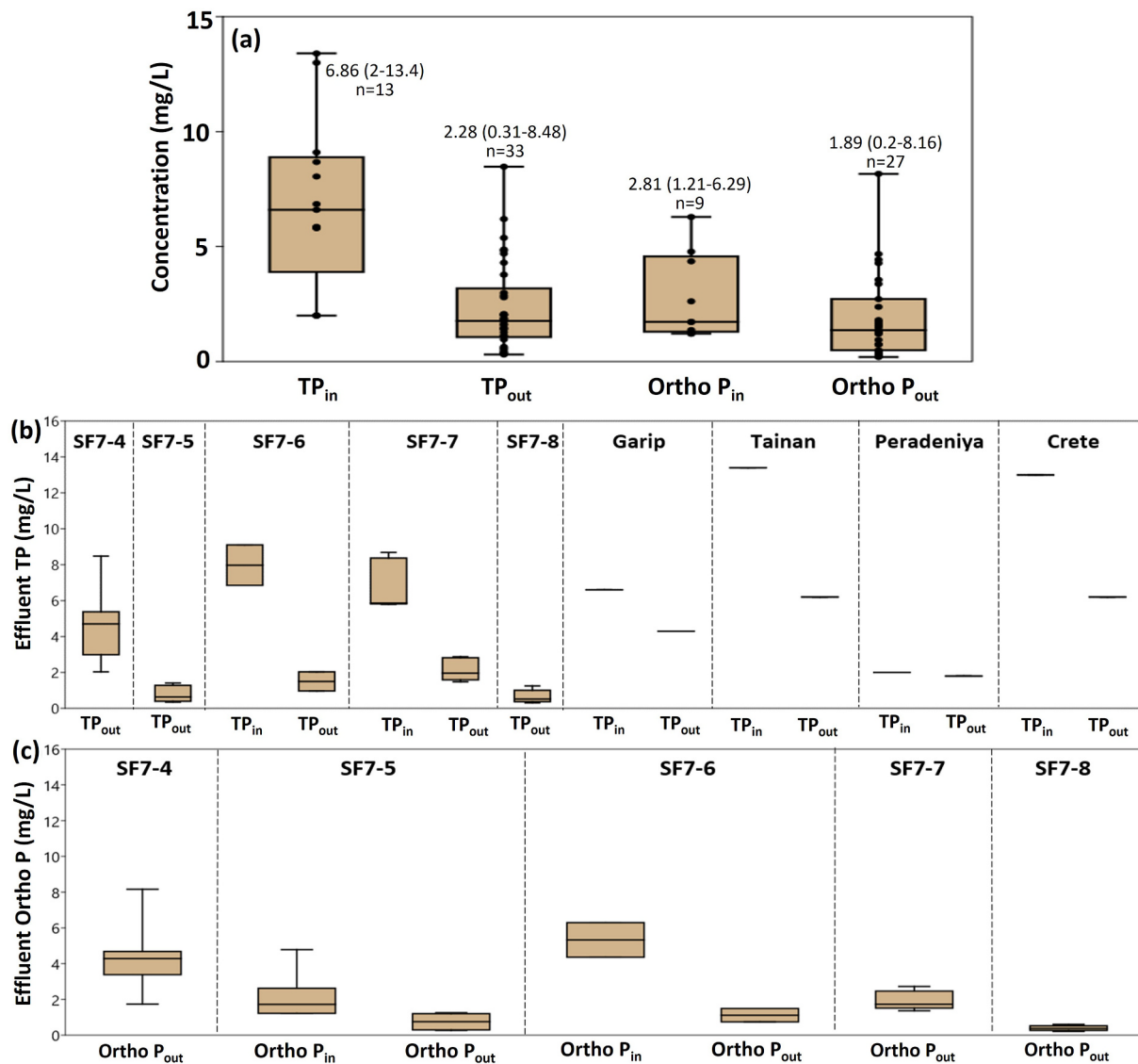
Fig. 3. The average concentrations of influent total phosphorus (TP in ), influent orthophosphate (Ortho P in ), effluent total phosphorus (TP out ), and effluent orthophosphate (Ortho P out ) of the SF TWs for secondary treatment (a); annual average influent and effluent concentrations of TP (b) and ortho P (c) from each secondary treatment wetland. The corresponding system names in the X-axis can be found in Table S1. Error bars represent the minimum and maximum mean values in each dataset and n represents the number of annual average value datapoints from all systems.
