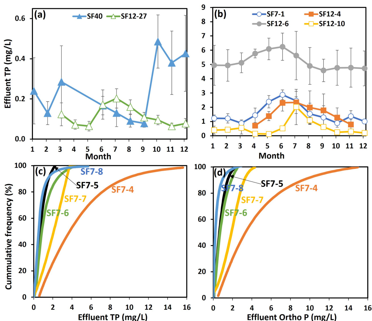
Fig. 5. Effluent total phosphorous (TP) concentrations from SF TWs for tertiary treatment based on monthly averages, (a) with targeted upstream P removal, (b) without targeted upstream P removal. The cumulative probability curves of the effluent TP (c) and Ortho P (d) from five secondary treatment systems. More vertical lines are indicative of inherently robust systems.
