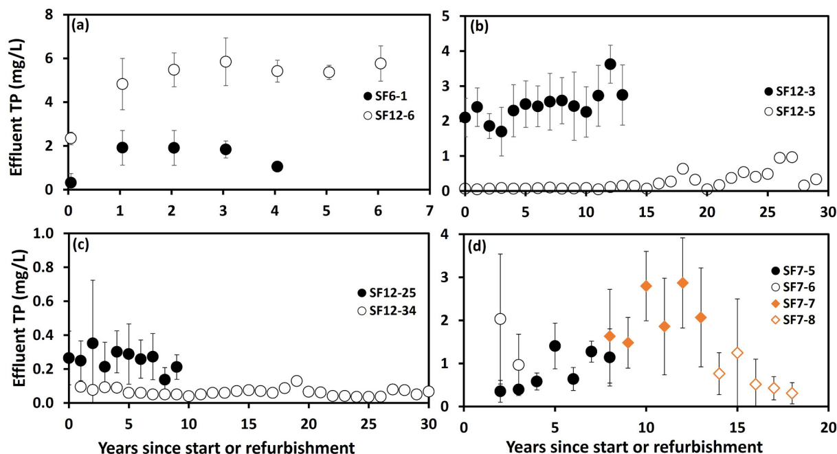
Fig. 4. Annual average effluent TP concentrations of (a) two systems with an increase between commissioning and their first year of operation from tertiary SF systems without targeted upstream P removal. Two examples of the other 30 tertiary SF systems without targeted upstream P removal (b), two examples of 12 tertiary SF systems with targeted upstream P removal (c), and four secondary treatment systems (d) showed no clear pattern for year-on-year changes. The error bars in the data indicate the standard variation of the annual values. The system names are shown in Table S1 .
