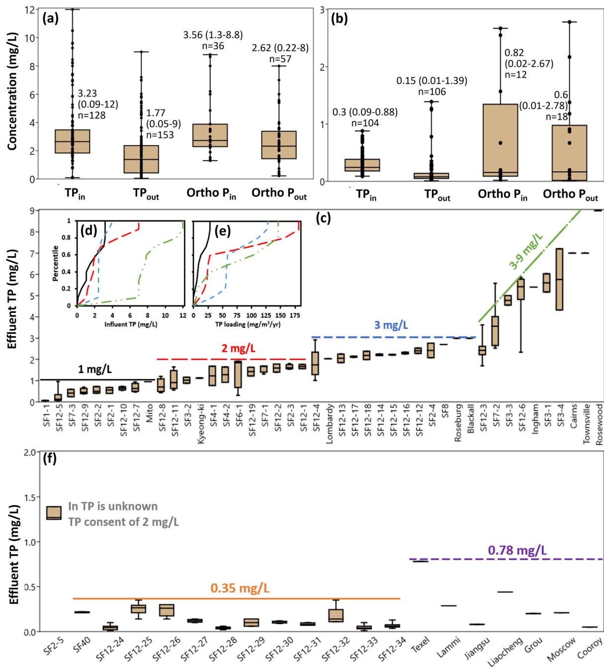
Fig. 2. Annual average concentrations of influent total phosphorus (TPin), influent orthophosphate (Ortho Pin), effluent total phosphorus (TPout), and effluent orthophosphate (Ortho Pout) of the SF TWs for tertiary treatment without (a) and with targeted upstream P removal (b). In the box-whisker plots, descriptive error bars represent the whole range of the data. Values above each box shows the mean (min-max). N represents the number of data points. (c) TPout from each SF TW for tertiary treatment without targeted upstream P removal; the percentile distribution of TPin (d) and TP loading (e) based on the four ranges of TPout identified in (c). (f) TPout from the systems for tertiary treatment with targeted upstream P removal. Data under orange solid line represents systems with long-term monitoring data; data under purple dash line represent informative data from literature for comparison purposes. The labelling of systems in the X-axis and associated grouping can be found in Table S1.
