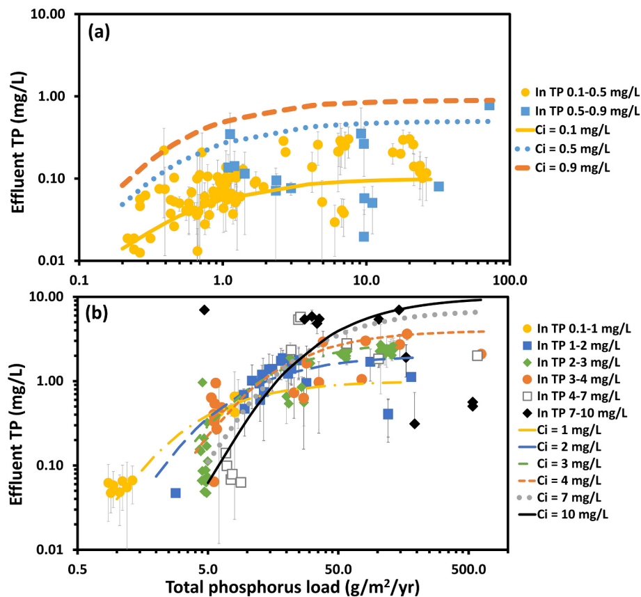
Fig. 6. Outlet TP concentration response to inlet TP loading of (a) 18 SF TWs for tertiary treatment with targeted upstream P removal and (b) 30 SF TWs for tertiary treatment without targeted upstream P removal. Symbols represent annual average data. In (a), n = 88 for the 0.1–0.5 mg/L inlet range and n = 14 for the 0.5–0.9 mg/L inlet range. Lines represent bounding model calculation for k = 6.79 m/yr, C^* = 0.006 , and P = 4 . In (b), n = 13 for the 0–1 mg/L inlet range, n = 24 for the 1–2 mg/L inlet range, n = 47 for the 2–3 mg/L inlet range, n = 19 for the 3–4 mg/L inlet range, n = 12 for the 4–7 mg/L inlet range, n = 12 for the 7–10 mg/L inlet range. Lines represent bounding model calculation for k = 5.31 m/yr, C^* = 0.006 , and P = 4 .
