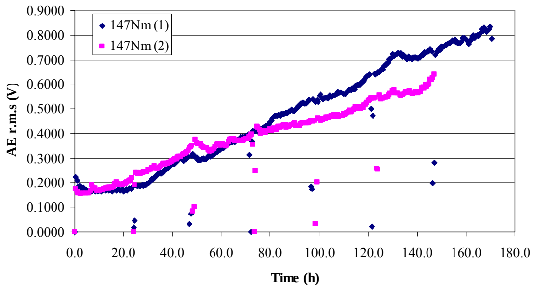
Figure 19 AE r.m.s. against operating time at 147 Nm; 745 rpm
