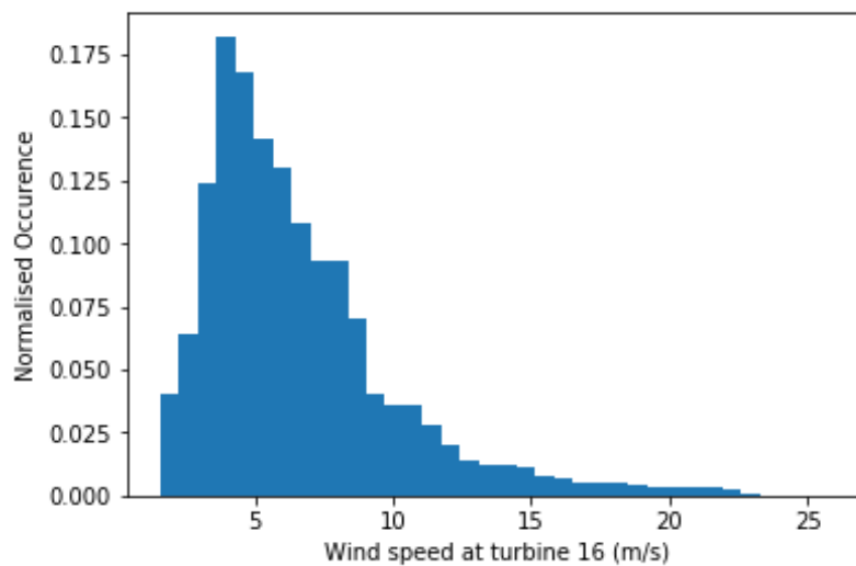
Figure 6. Histogram of recorded wind speed, turbine 16
