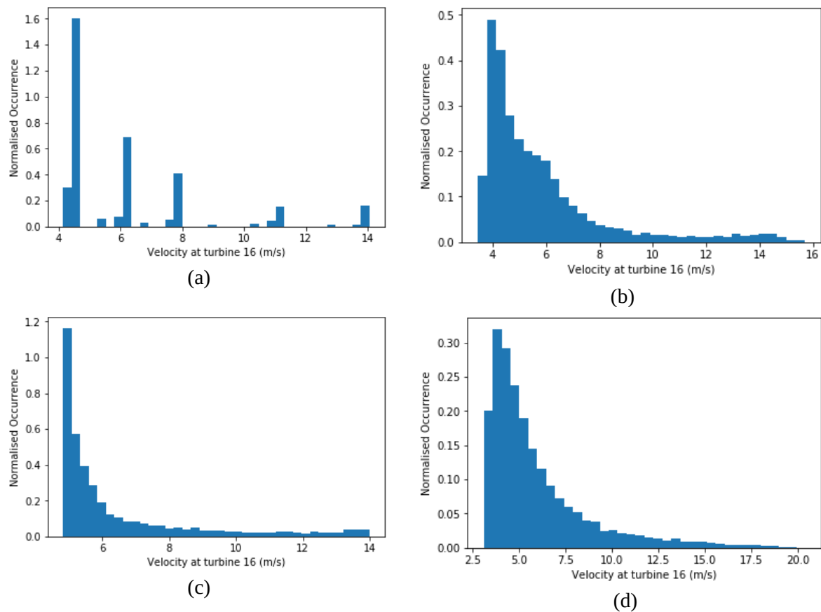
Figure 5. Probability distribution functions for the velocity at turbine 16 for (a) RF, (b) GP, (c) SVR and (d) ANN respectively.
