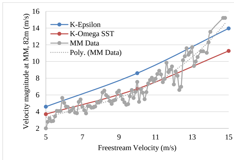
Figure 2. Comparison of turbulence models with met mast data.
