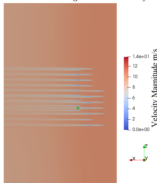
Figure 1. Velocity-magnitude field from steady state actuator disk model, met mast location denoted in green
