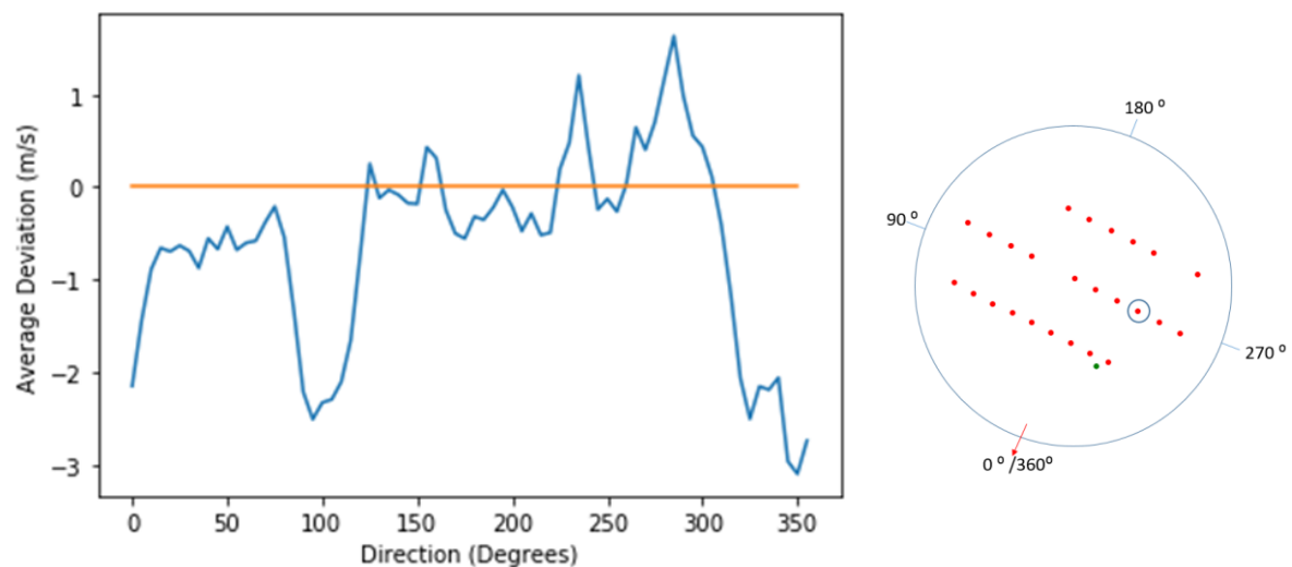
Figure 4. Wind velocity deviation from freestream velocity by angle at the met mast (left) and a map of the wind farm (right), turbines in red and met mast in green, turbine 16 circled in blue, red arrow shows wind direction of 0 degrees.
