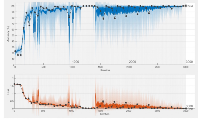
Fig. 3. RNN Training Performance: accuracy and loss function over training iterations.
