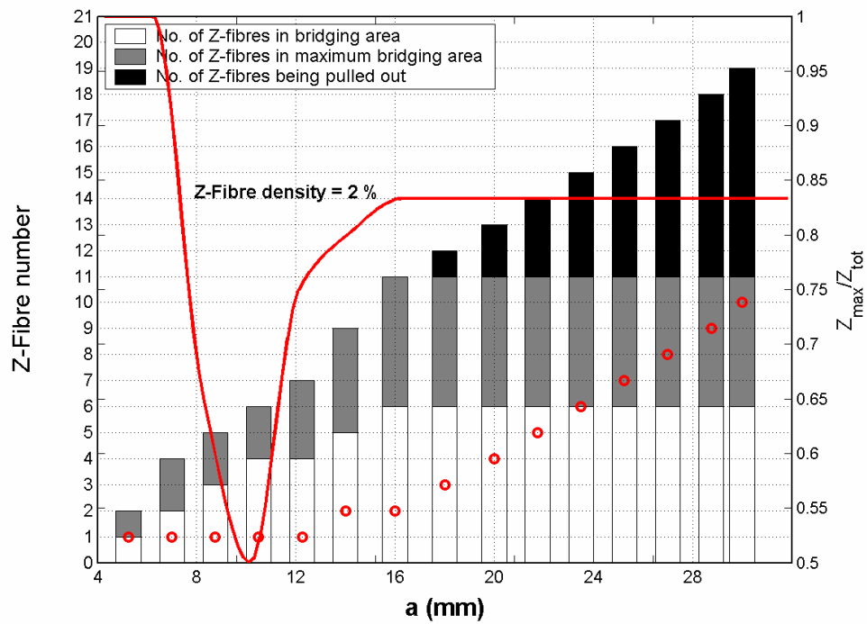
Fig. 9 Z-fibre bridging process during delamination growth for a 2% z-pinned DCB showing the numbers of z-pins involved in the different stages (bar-chart), M_{\max} location (o), z-fibre ratio in \Phi_{\max} region (—).
