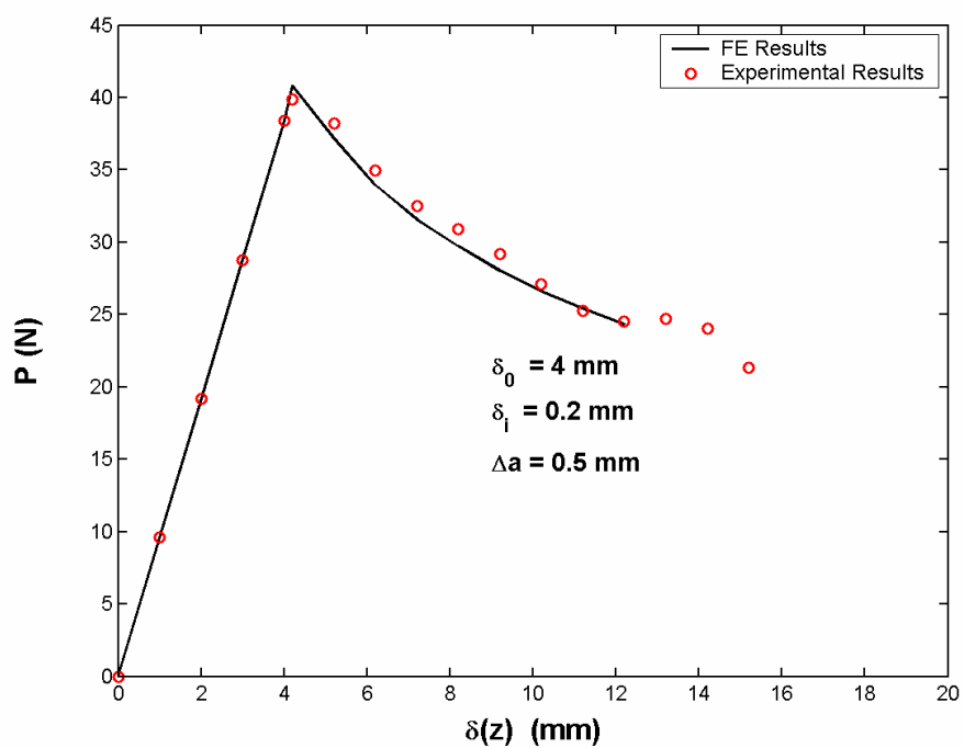
Fig. 5 Load-displacement relation for unpinned DCB (control case) – numerical vs. experimental results.
