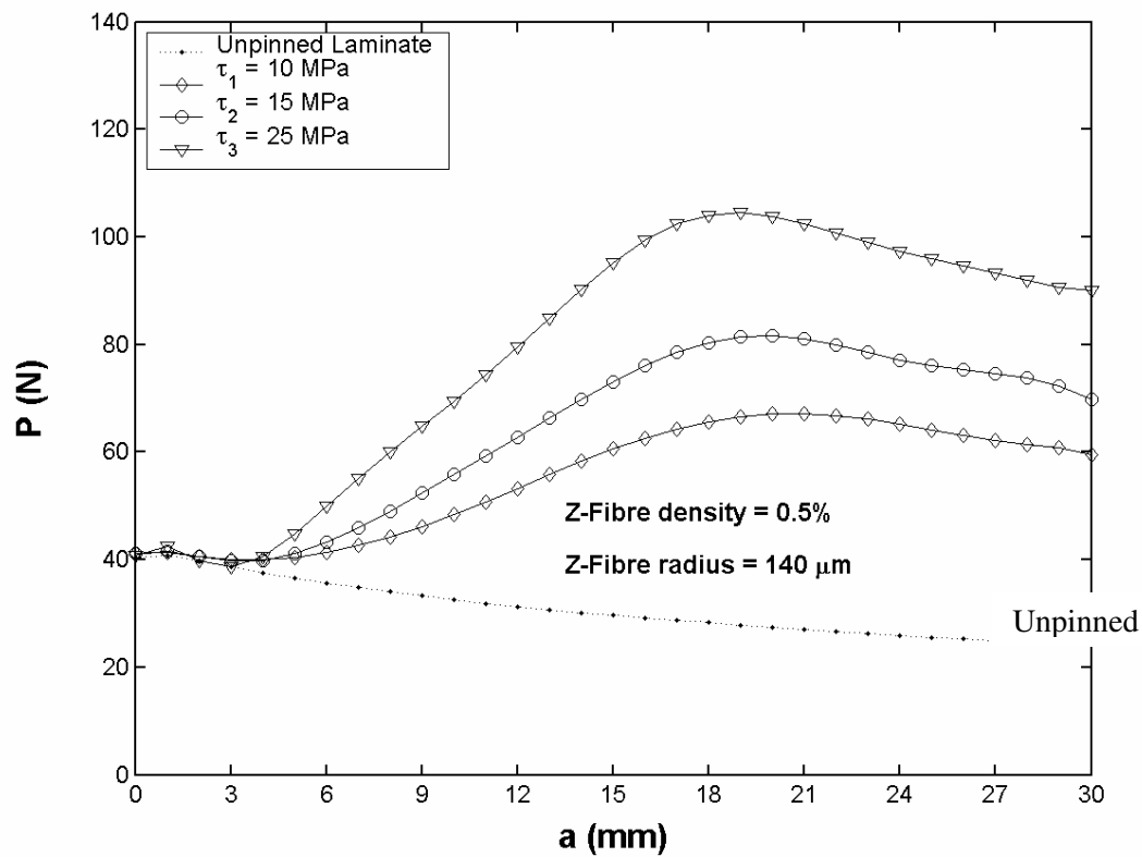
Fig. 13 Load vs. delamination length: effect of frictional stress between z-fibre and laminate.
