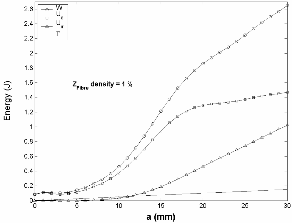
Fig. 16 Energy balance during delamination and z-fibre bridging process (z-pin radius r_1 ).
