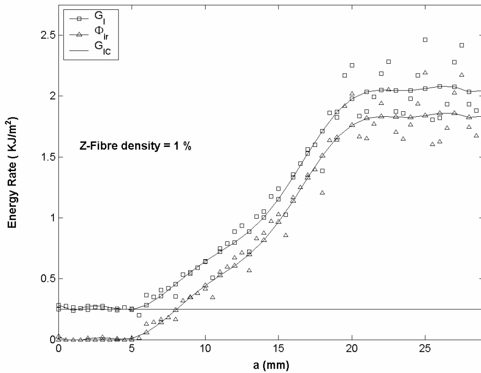
Fig. 17 Energy rates during delamination and z-fibre bridging process (z-pin radius r_1 ).
