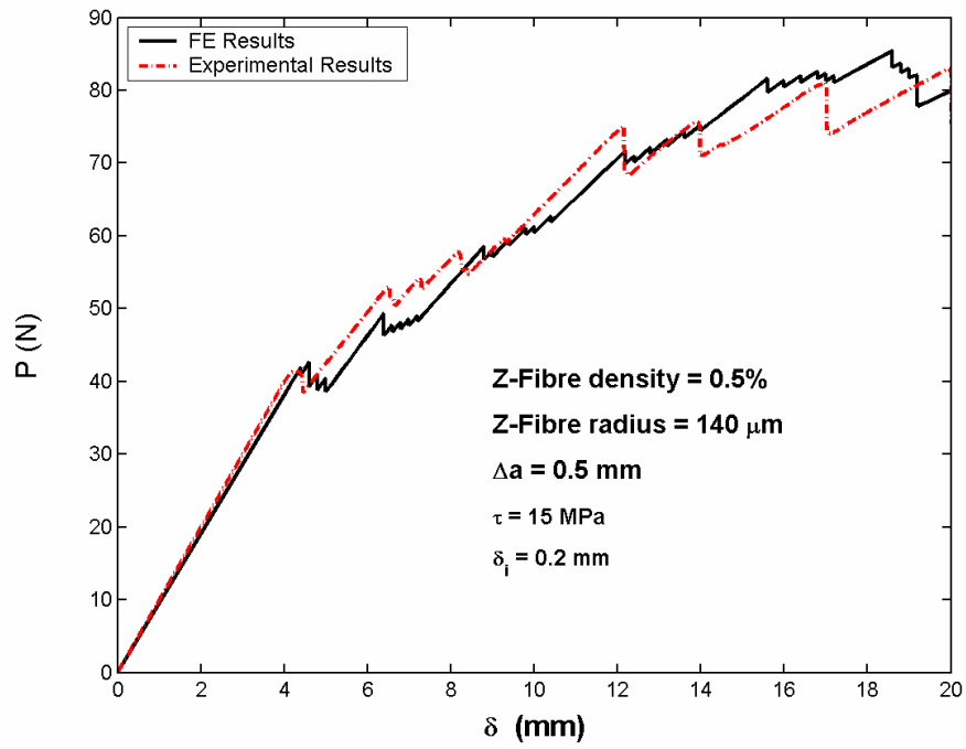
Fig. 6 Load-displacement curves for z-pinned DCB – Numerical vs. experimental results.
