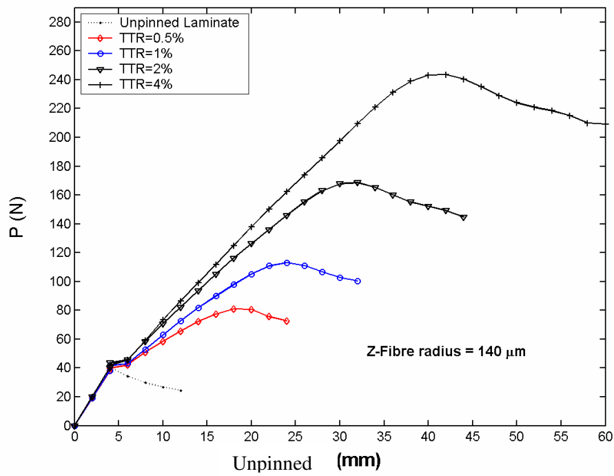
Fig. 10 Computational P - \delta curves for different z-fibre densities and comparison with un-pinned case.
