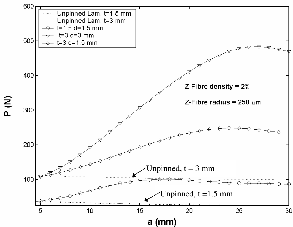
Fig. 15 Load vs. delamination length: effect of laminate thickness & z-pin insertion depth.
