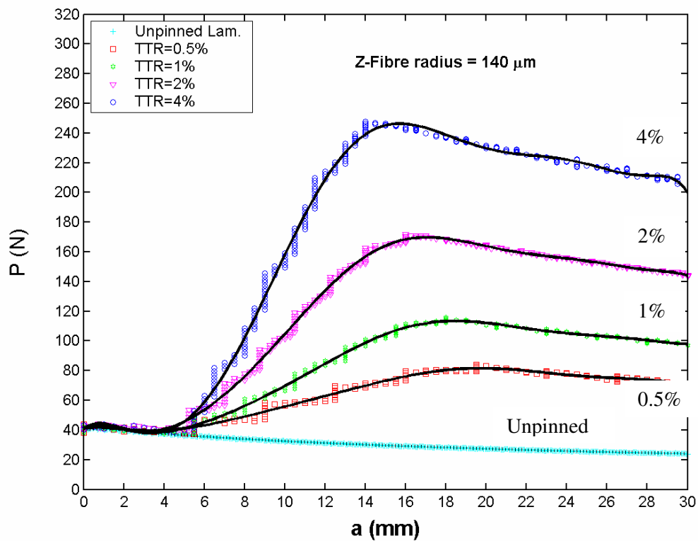
Fig. 11 Load vs. delamination length for different z-pin densities and comparison with unpinned case. FE results (discrete symbols); polynomial interpolation (smooth lines).
