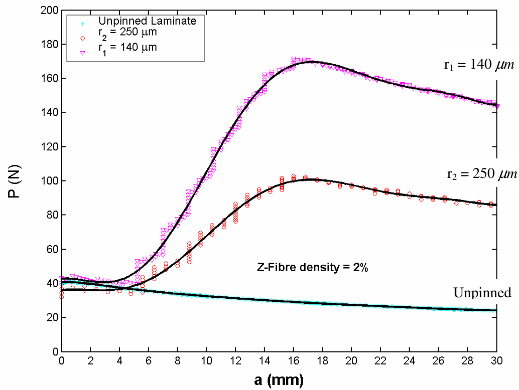
Fig. 12 Load vs. delamination length: z-pin diameter effect.
