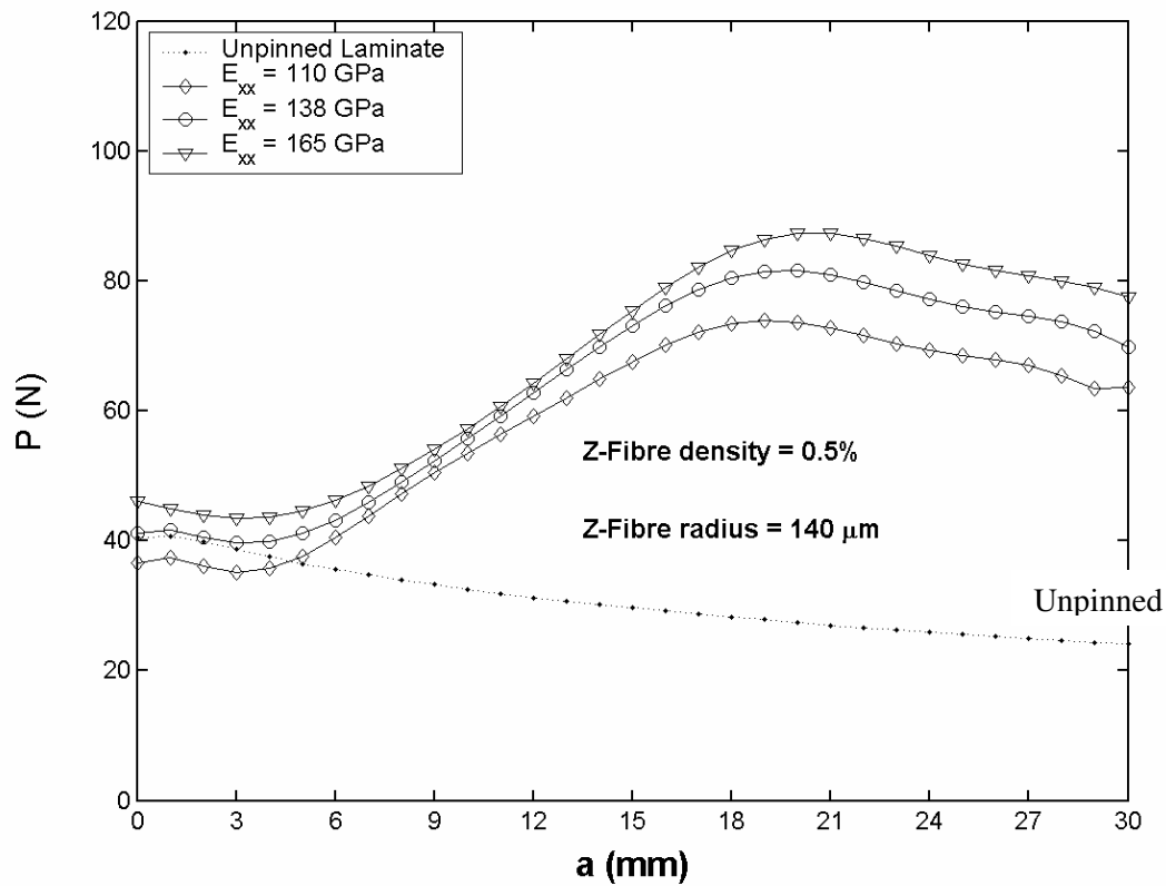
Fig. 14 Load vs. delamination length: effect of laminate flexural rigidity (0.5% z-pin density and 0.28 mm z-fibre diameter)
