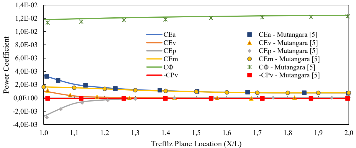
Fig. 14: Comparison of subsonic Power Balance coefficients for F-57 body.
