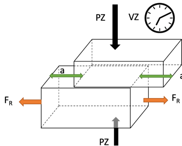
Fig. 1. Methods of wood welding where PZ is welding pressure, VZ is welding time, F_R is friction force, and a is amplitude of vibratory movement (Horman et al. 2016)
