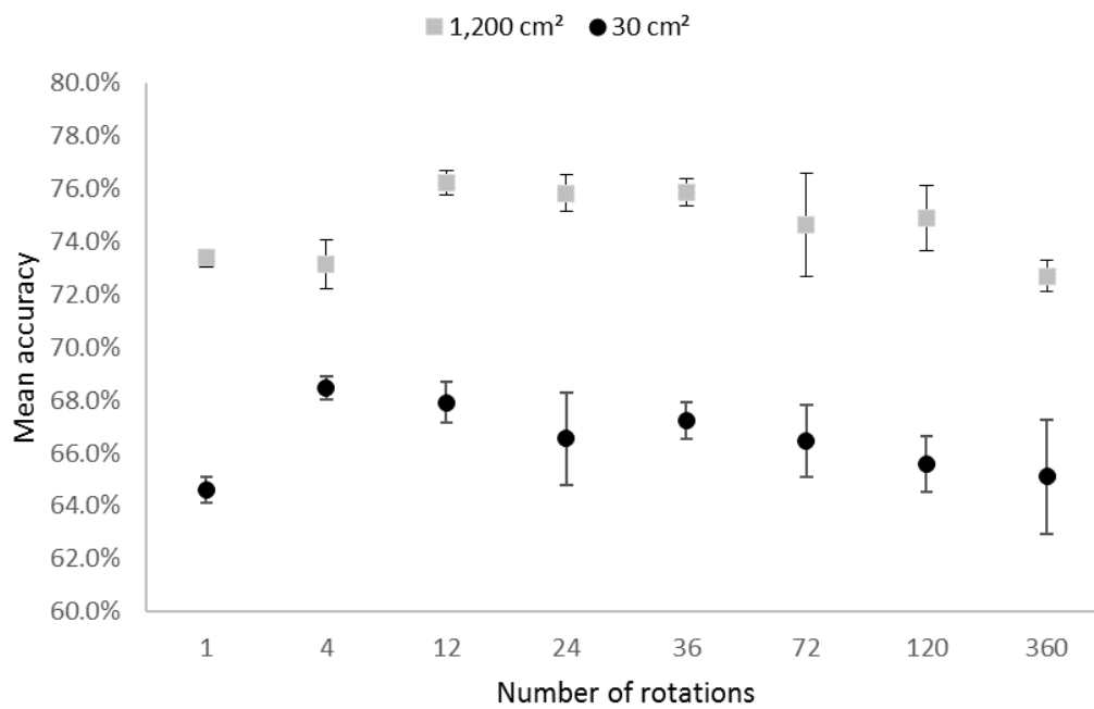
Fig. A7. Effects of using software rotations to increase the number of training images, for different crop sizes. The vertical bars denote standard deviation.
