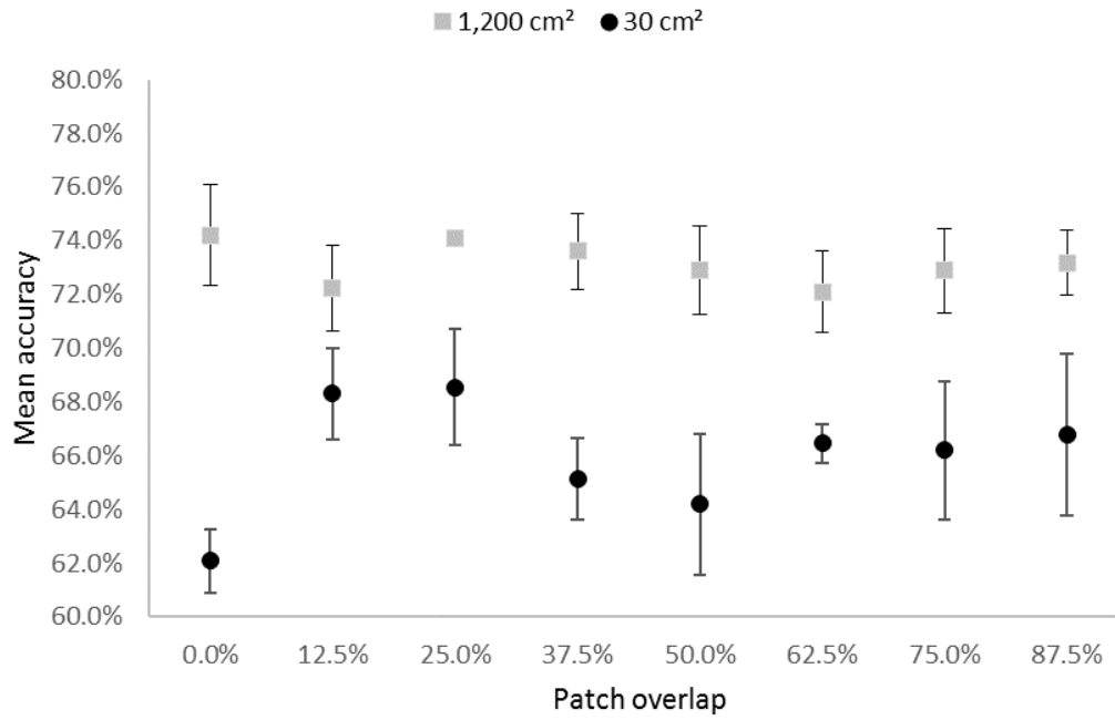
Fig. A8. Effects of using different patch overlapping factors to increase the number of training images, for different crop sizes. The vertical bars denote standard deviation.
