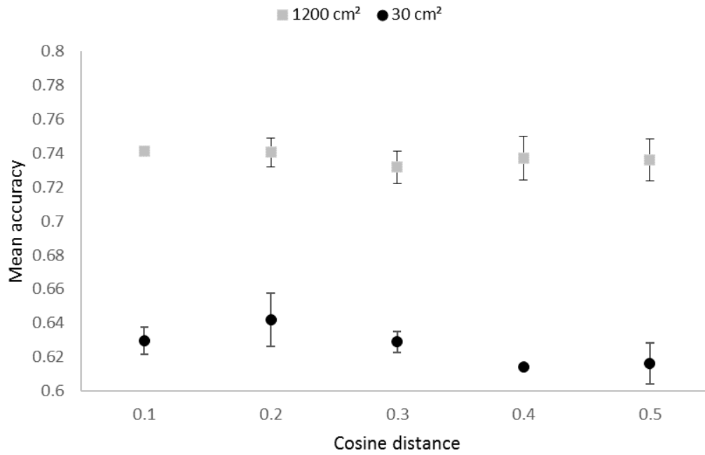
Fig. A6. Effects of using different cosine distances between training images, for different crop sizes. The vertical bars denote standard deviation.
