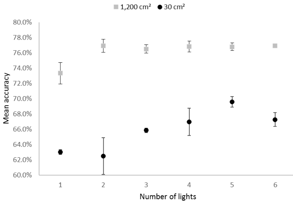
Fig. A9. Effects of using different number of lights to increase the number of training images, for different crop sizes. The vertical bars denote standard deviation.
