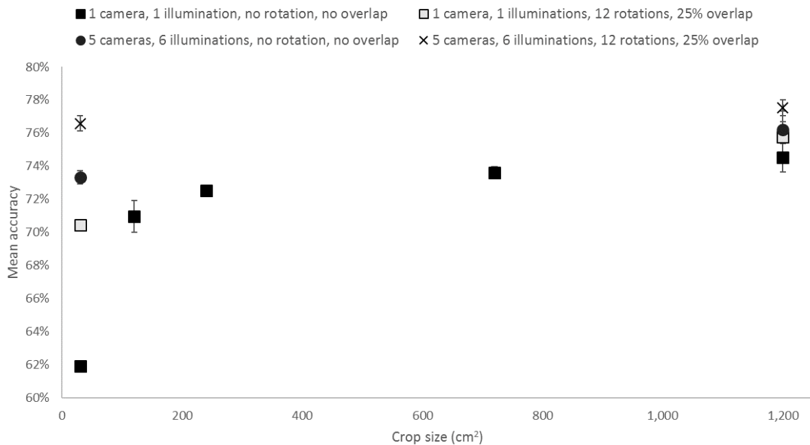
Fig. 4. Combined effects of different techniques when applied to different crop sizes. Vertical bars indicate standard deviation.
