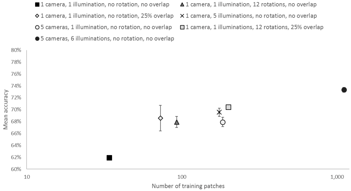
Fig. 2. Effects of different techniques to increase the number of training patches and improve accuracy when using 30 cm 2 crops, on a log-10 scale. Vertical bars indicate standard deviation.
