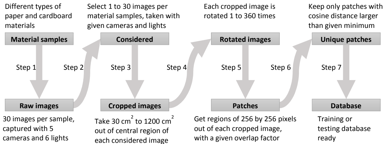
Fig. 1. Steps taken to create the training and testing databases.
