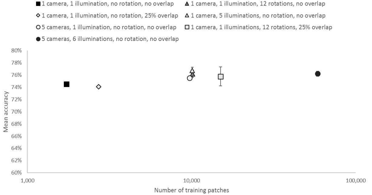
Fig. 3. Effects of different techniques to increase the number of training patches and improve accuracy when using 1,200 cm 2 crops, on a log-10 scale. Vertical bars indicate standard deviation.
