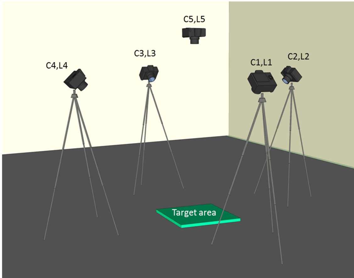
Fig. A1. Schematics depicting the image capture hardware configuration which includes 5 cameras (C1 – C5) and 5 lights (L1 – L5). The lights (not shown) are located next to the cameras, also pointing towards the target area.
