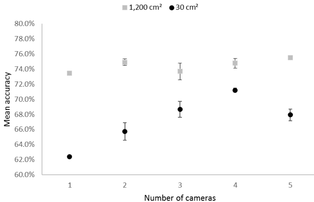
Fig. A10. Effects of using different number of cameras to increase the number of training images, for different crop sizes. The vertical bars denote standard deviation.
