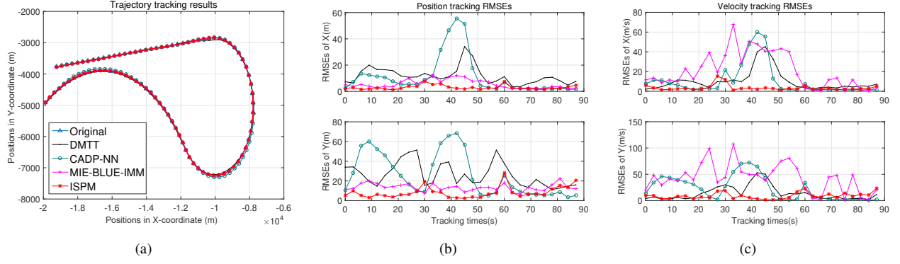
Fig. 19. Tracking results of low-maneuvering trajectory with \sigma_\theta = 2 \times 10^{-3} \text{rad} and \sigma_d = 4\text{m} .
