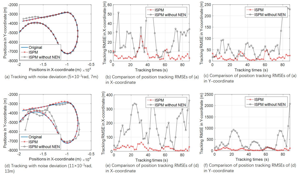
Fig. 26. Ablation experiments.
