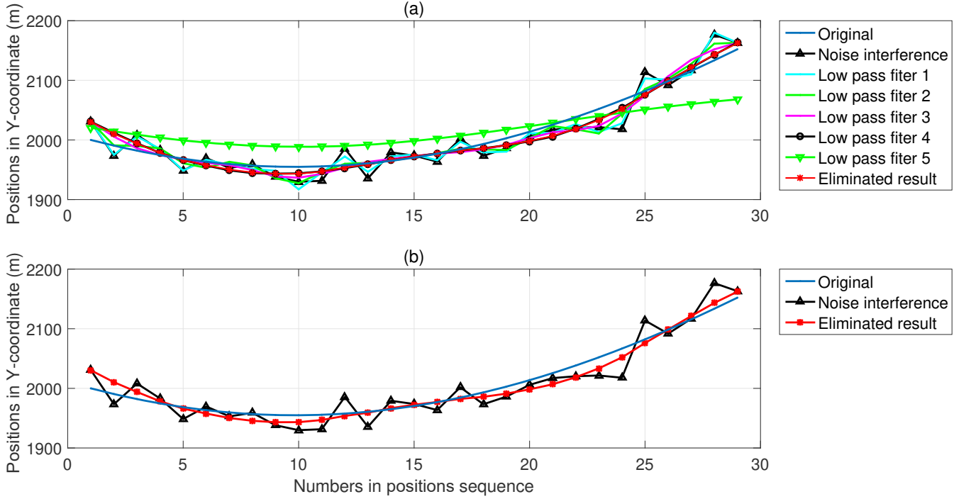
Fig. 10. Noise elimination results.
