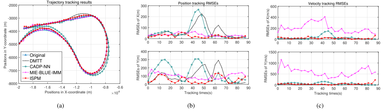
Fig. 22. Tracking results of low-maneuvering trajectory with \sigma_\theta = 11 \times 10^{-3} \text{rad} and \sigma_d = 13 \text{m} .
