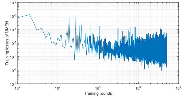
Fig. 15. MMEN training with noise-eliminated input data.
