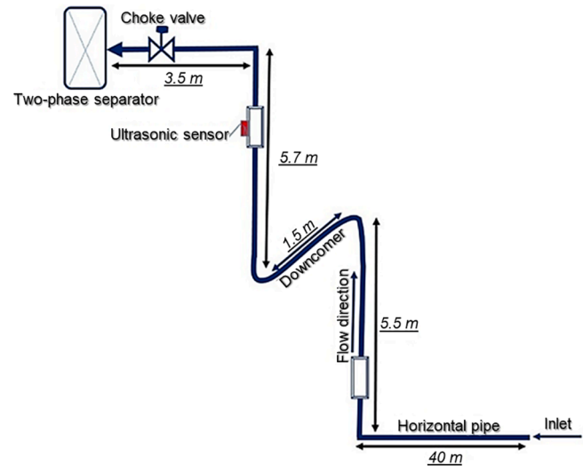
Fig. 3. The schematic diagram of the S-shape riser.
