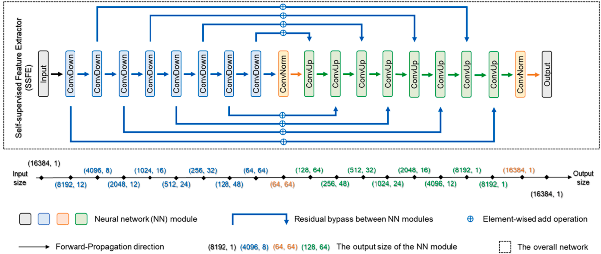
Fig. 5. The network structure of the proposed SSFE.
