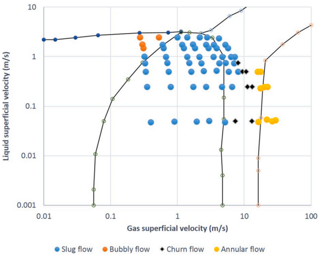
Fig. 4. The flow regime diagram.
