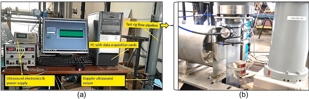
Fig. 2. The photos of the two-phase flow test riser.
