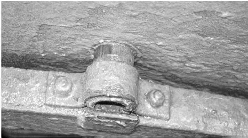
Figure 61 'U' strap for retaining through rod to support structure
