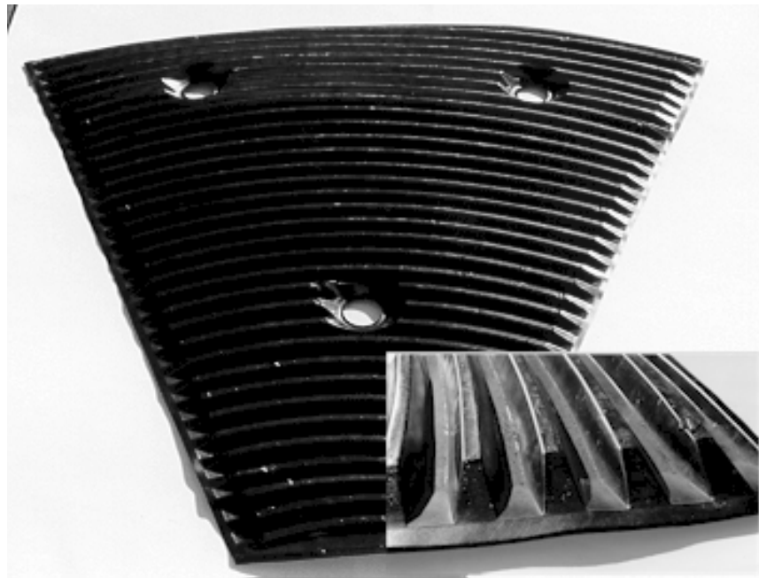
Figure 19 Polymer media panel, type 3: Layout
