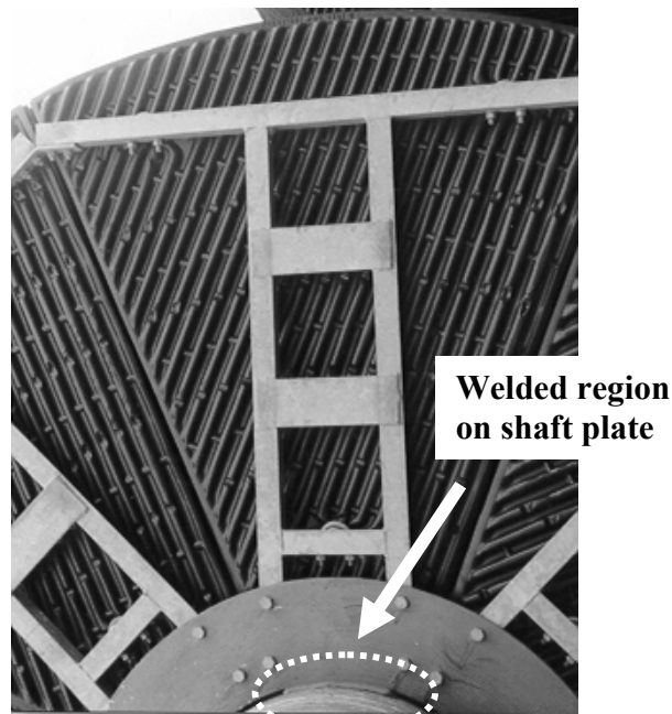
Figure 56 RBC design arrangement to improve bending resistance
