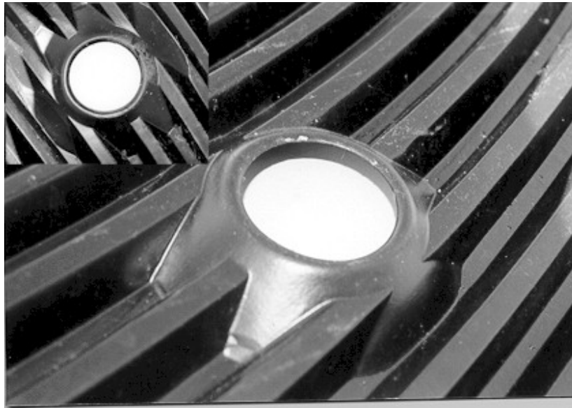
Figure 29 Improved strength of hole in media panel
