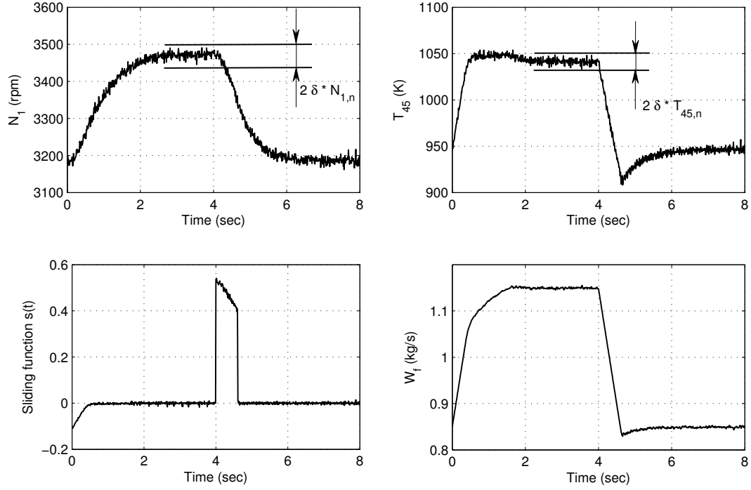
Figure 7: Fan speed, exhaust gas temperature, sliding function, and fuel flow mass responses in the final simulation.
