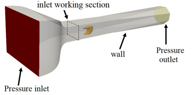
(a) LLF-DNW wind tunnel sub-domain. The rig surface is included for reference of the overall size
