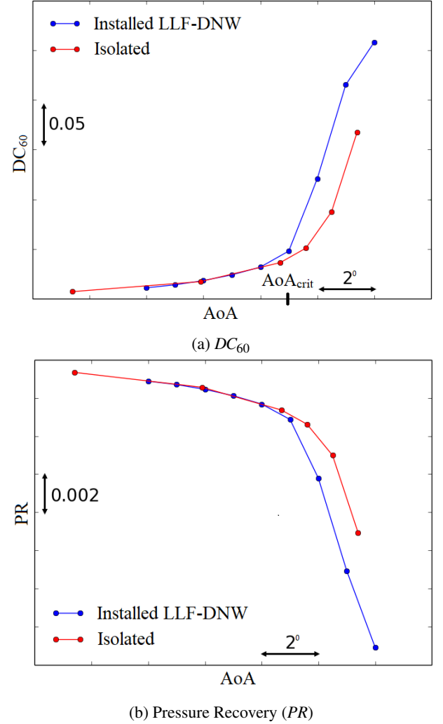
Figure 7: Comparisons of intake distortions metrics between installed LLF-DNW and isolated configurations at MFCR \approx 1.6
