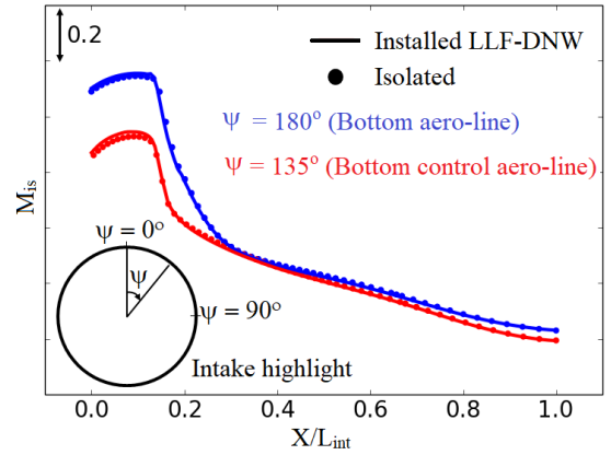
Figure 5: Comparison of isentropic Mach number along the intake bottom ( \psi = 180^\circ ) and bottom-control ( \psi = 135^\circ ) aero-lines between the isolated and installed LLF-DNW at MFCR \approx 1.6 and AoA = AoA_{crit} - 1^\circ
