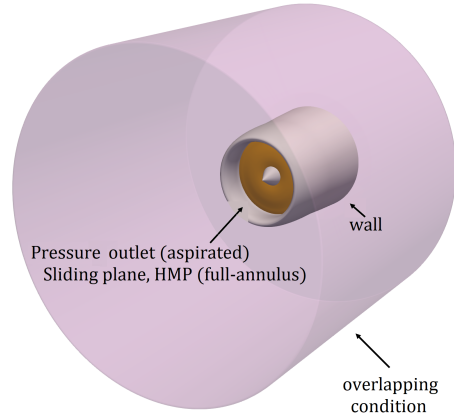
(c) Intake sub-domain
