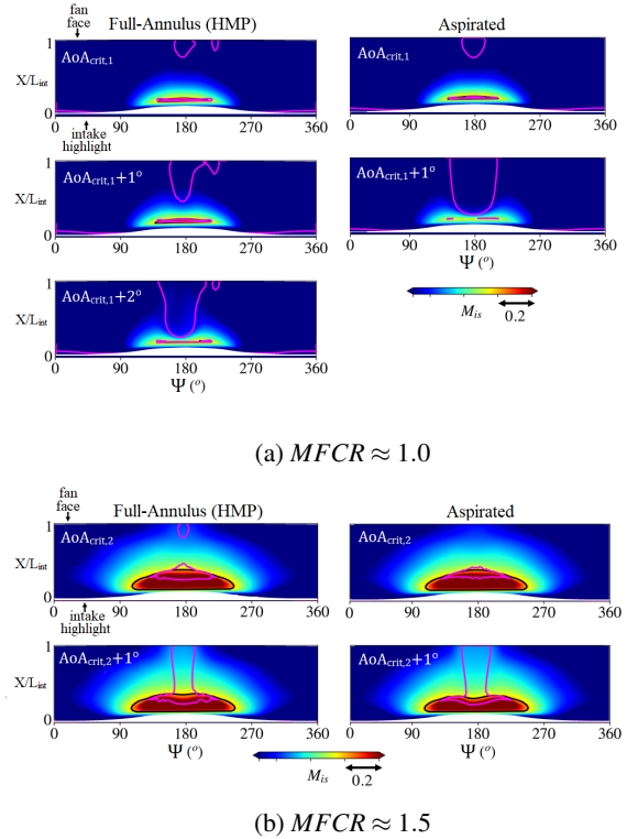
Figure 12: Unwrapped surfaces of the intake colored by isentropic Mach number distribution. Black iso-lines are for M_{is} = 1 and pink isolines are for axial wall shear stress of 0
