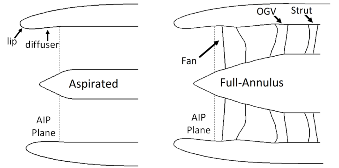
Figure 1: Overview of intake modelling: Aspirated intake (left) and fan-intake coupled (right)
