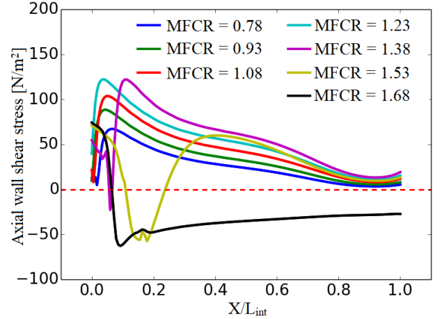
(b) Axial wall shear stress
