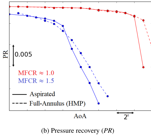
Figure 11: Impact of fan-suppression on intake distortion metrics
