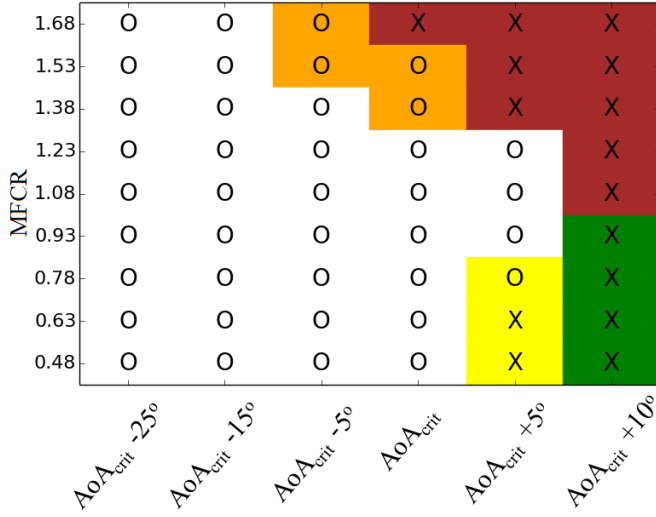
Figure 9: Categorization of the intake flow characteristics with the proposed taxonomy across the MFCR-AoA aerodynamic design space. White color refers to attached flow. The symbols \circ and \times are for DC_{60} < DC_{60,ref} and DC_{60} > DC_{60,ref} , respectively. The same color code is used in Fig. 8
