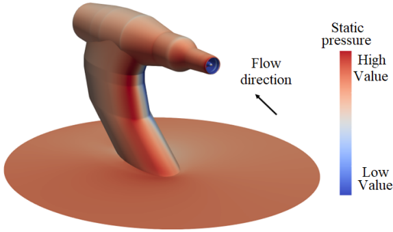
Figure 4: Example of the CFD solution for the installed aspirated configuration (rig and intake sub-domains) at M = 0.25 , AoA = AoA_{crit} - 1^\circ and MFCR \approx 1.6
