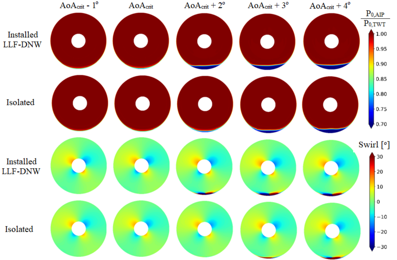
Figure 6: Effect of incidence angle on total Pressure Recovery (PR) and swirl distortion at the AIP for the installed LLF-DNW and isolated configurations at MFCR \approx 1.6
