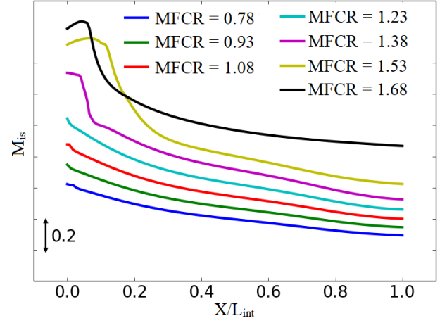
(a) Isentropic Mach number
