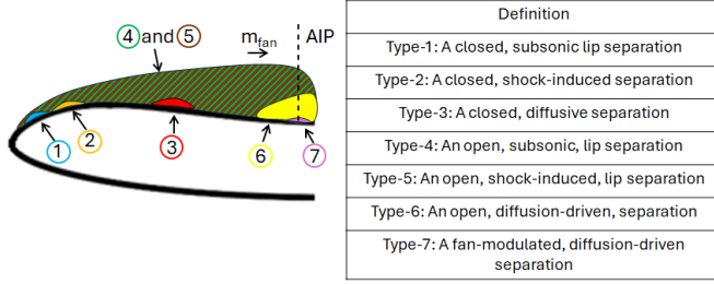
Figure 8: Flow separation taxonomy to characterise the intake characteristics. The same color code is used in Fig. 9
