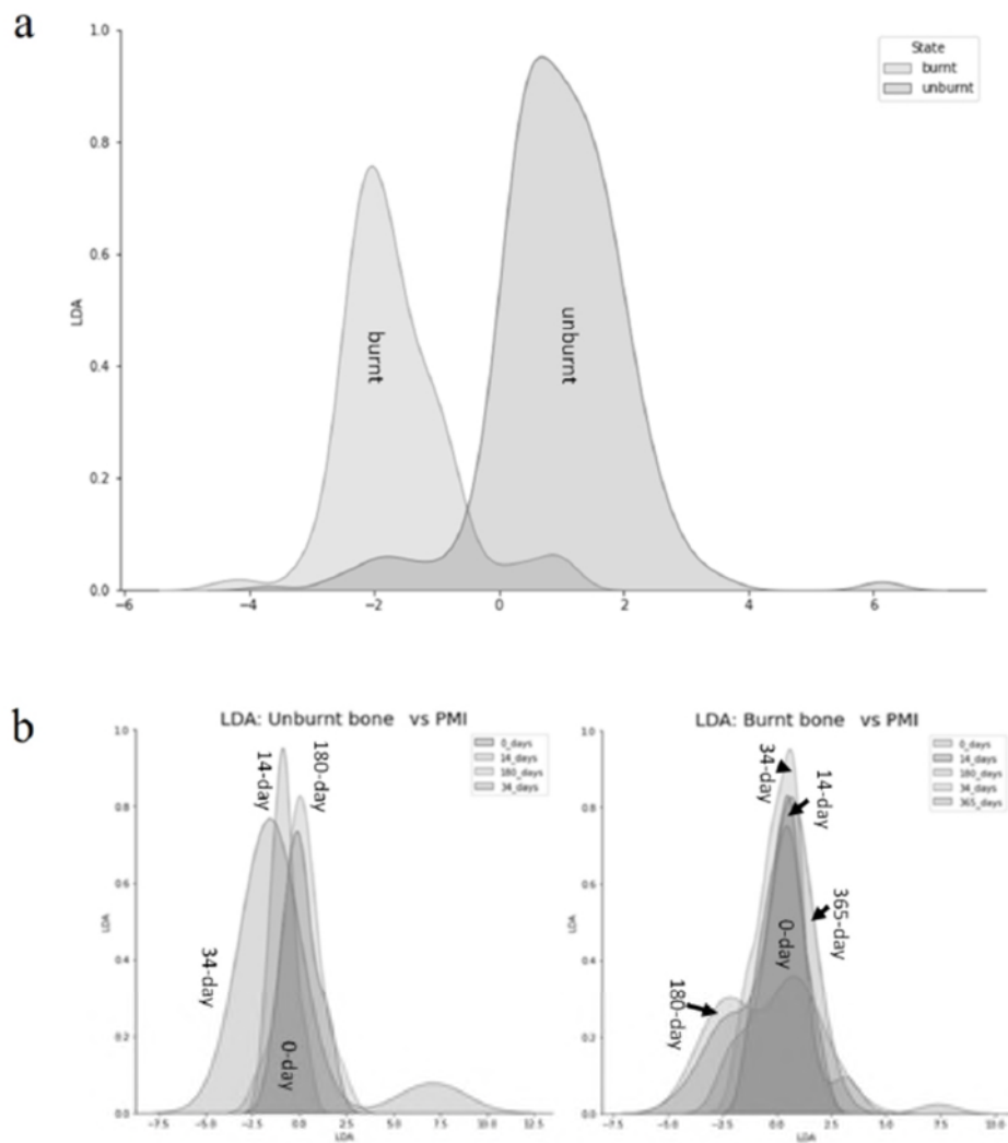
Fig. 6 – Linear discriminant analysis (LDA) on the EMPA dataset. A: Separation of unburnt and burnt bone by LDA. Contributions: 'Al 2 O 3 ': 0.244, 'CaO': -6.882, 'Cl': 3.216, 'FeO': 0.07, 'K 2 O': 0.607, 'MgO': -1.036, 'MnO': -0.056, 'Na 2 O': -0.545, 'P 2 O 5 ': -3.97, 'SiO 2 ': -0.902, 'SrO': 0.199, 'Total': 13.08. B: Clusters created by LDA of the unburnt (left) and burnt (right) PMI groups.
