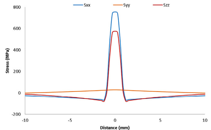
Fig. 12. Residual stress distributions in the three directions of space predicted numerically for weld 5.
