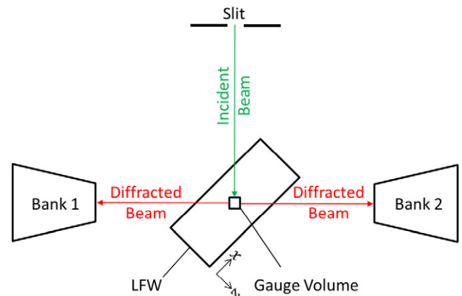
Fig. 3. Experimental set-up used with ENG-X diffractometer.
