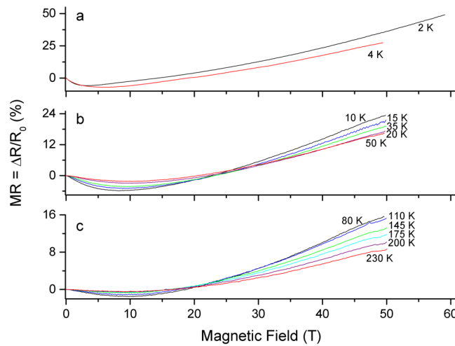
Figure 6. For clarity, the MR of the aligned CNT fiber is shown in three different temperature ranges: (a) 2–4 K, (b) 10–50 K, (c) 80–230 K. Note that the MR scales change on each plot. R_0 is the resistance at zero-field. Note that this response contrasts the level-off behavior of the unaligned SWCNT films.
