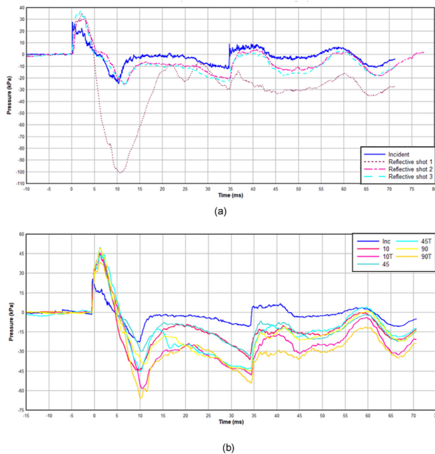
Figure 7. TS1 (a) Comfort pad P-t curves. (b) RetiCell mean P-t curves, those datasets incorporating the para-aramid in front of the foam denoted with 'T'.
