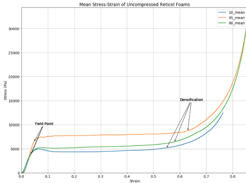
Figure 5. Mean Stress-Strain of 10, 45, and 90 PPI uncompressed Retigel foams, with clearly identifiable yield points used to calculate the Young's modulus from the gradient of the linear region.
