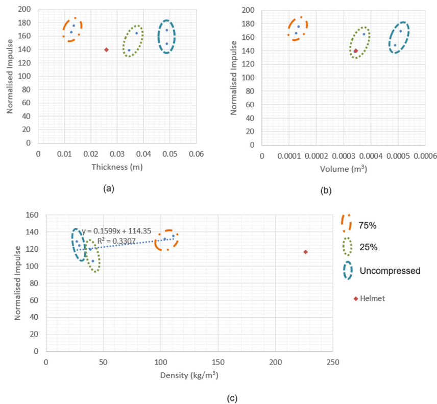
Figure 11. TS2 Effect of increasing (a) Thickness (b) Volume (c) Density of Retigel foams on normalised impulse.
