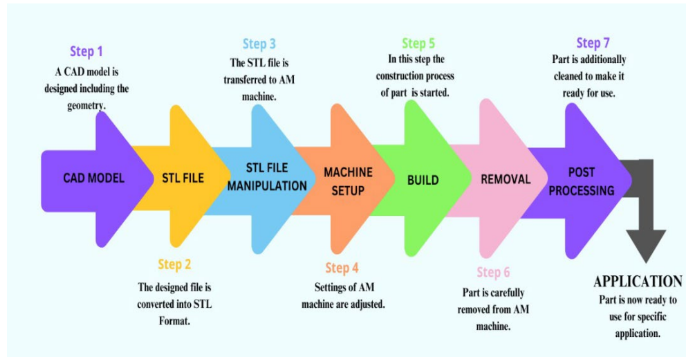
Figure 1.Overview of AM Process.
