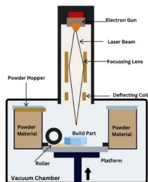
Figure 7. Pictorial Representation of the EBM.
