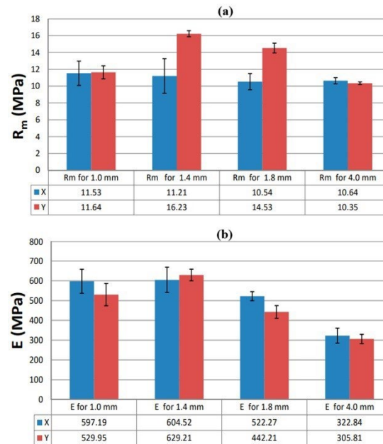
Figure 10. (a) Tensile strength ( R_m ) of PLA/bronze samples based on thickness and print direction (b). Elastic Modulus ( E ) of PLA/bronze samples based on thickness and print direction [11].
