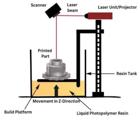
Figure 3. Pictorial Representation of the SLA.
