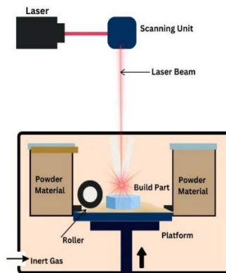
Figure 6. Pictorial Representation of the SLM
