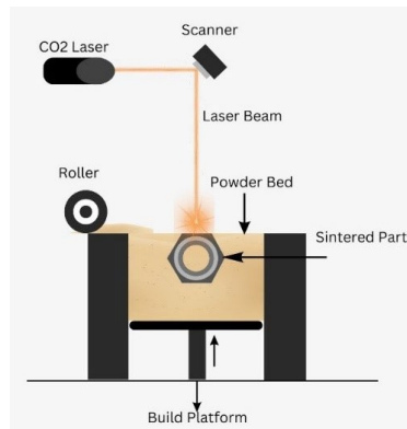
Figure 5. Pictorial Representation of the SLS
