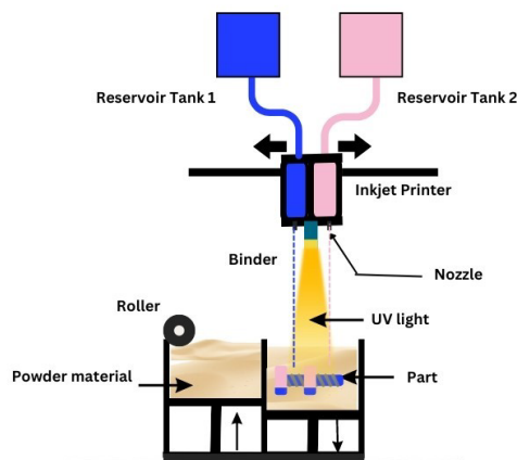
Figure 9. Pictorial representation of material jetting process.
