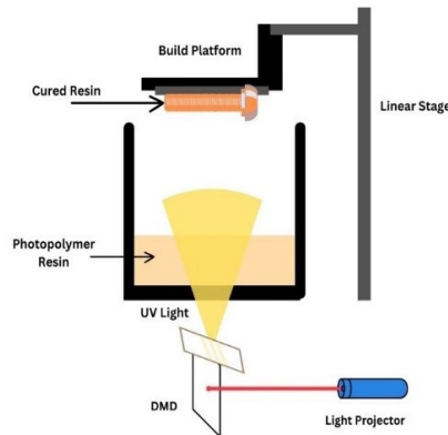
Figure 4. Pictorial Representation of the DLP.
