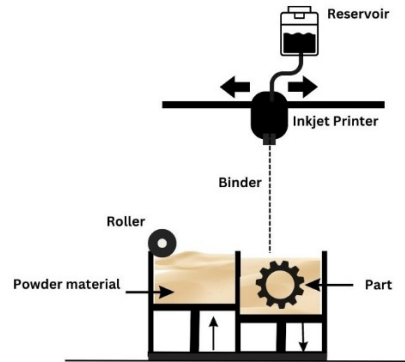
Figure 8. Pictorial representation of binder jetting process.
