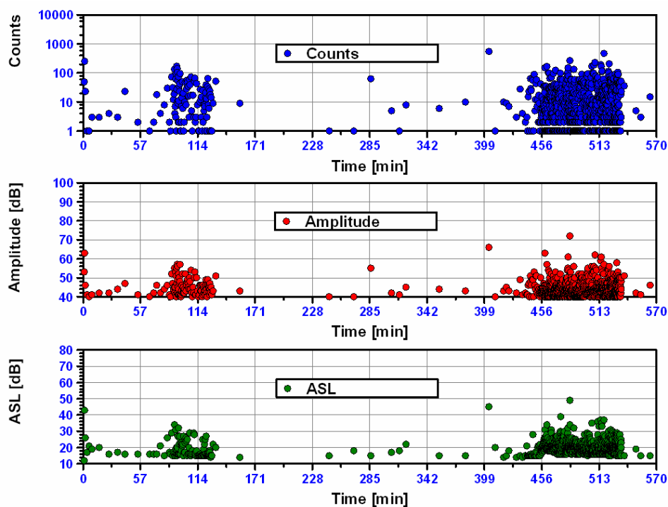
Figure 3 Classical AE parameters of counts, amplitude and ASL.
