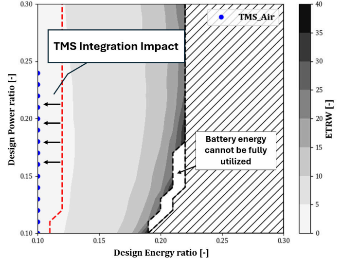
Figure 18. ETRW results - Single-Leg Mission; IPTMS optimization
