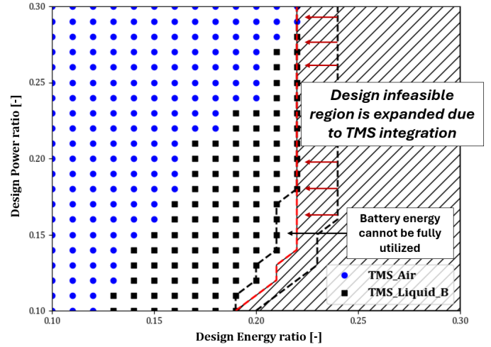
Figure 14. TMS design type - Single-Leg Mission; IPTMS optimization
