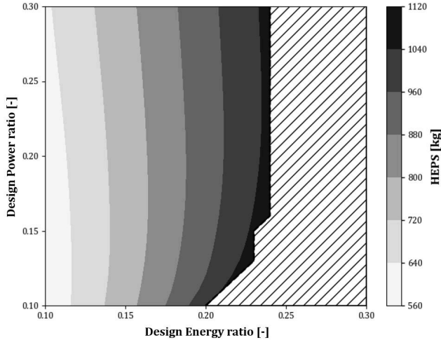
Figure 10. HEPS weight - Single-Leg Mission; PMS optimization
