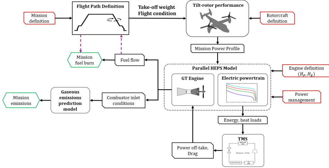
Figure 1. Multidisciplinary PHE rotorcraft framework with IPTMS
