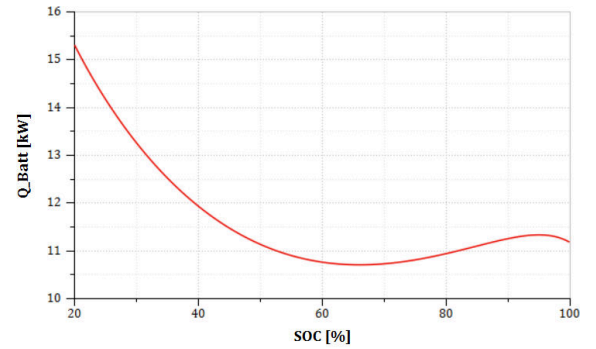
Figure 6. Battery heat load variation against its SOC
