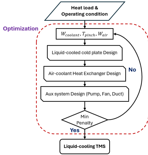
Figure 5. Liquid-cooling TMS design process
