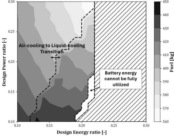
Figure 16. Fuel consumption - Single-Leg Mission; IPTMS optimization
