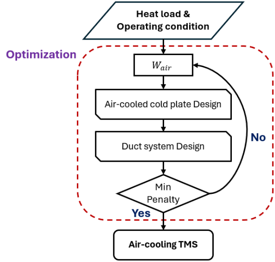
Figure 3. Air-cooling TMS design process
