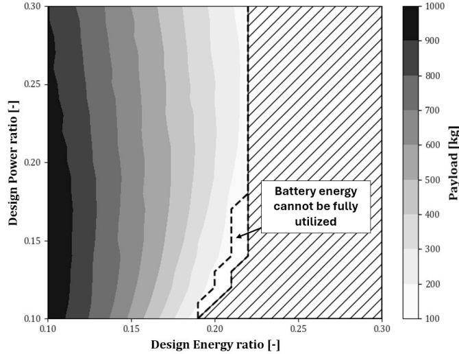
Figure 17. Payload - Single-Leg Mission; IPTMS optimization
