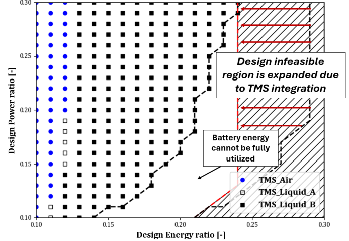
Figure 20. TMS design type - Double-Leg Mission; IPTMS optimization
