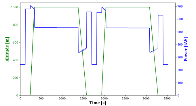
Figure 9. Altitude and power profile - Double-Leg mission
