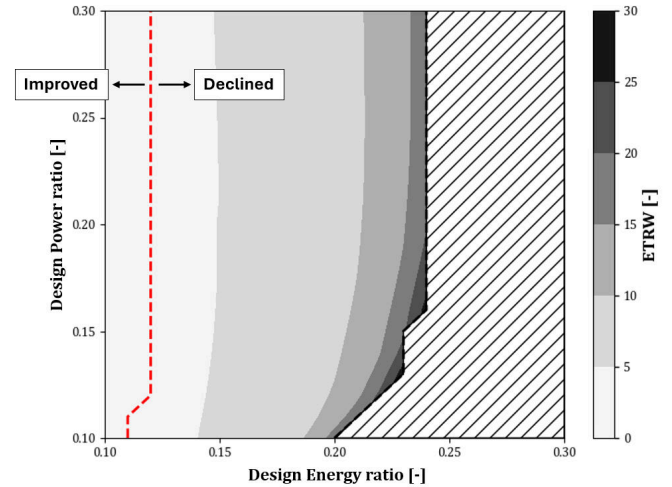
Figure 11. ETWR - Single-Leg Mission; PMS optimization
