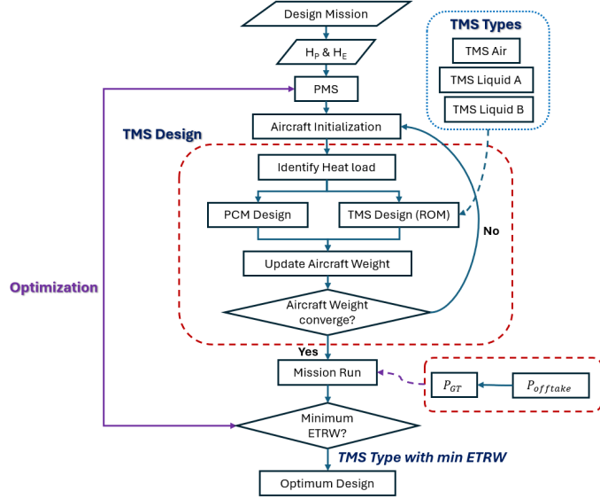
Figure 7. IPTMS optimization process
