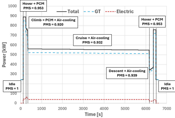
Figure 19. Optimal design case operation highlights – Single-Leg Mission
