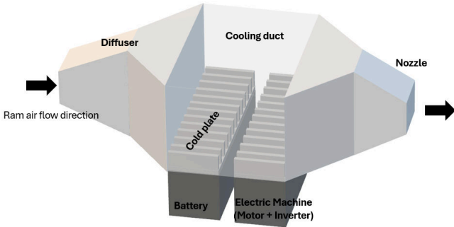
Figure 2. The air-cooling TMS design schematic
