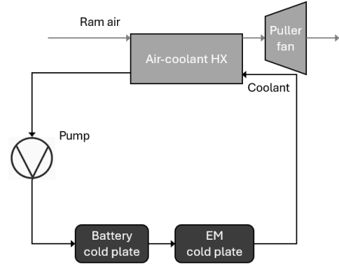
Figure 4. The liquid-cooling TMS design schematic
