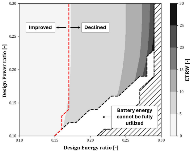
Figure 13. ETRW – Double-Leg Mission; PMS optimization
