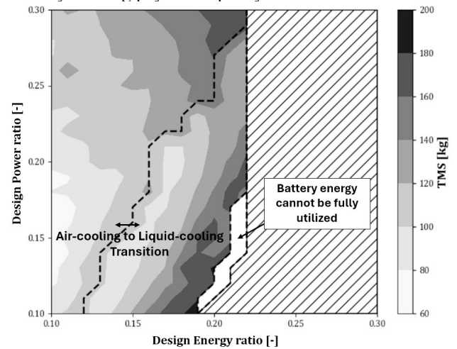
Figure 15. TMS weight - Single-Leg Mission; IPTMS optimization
