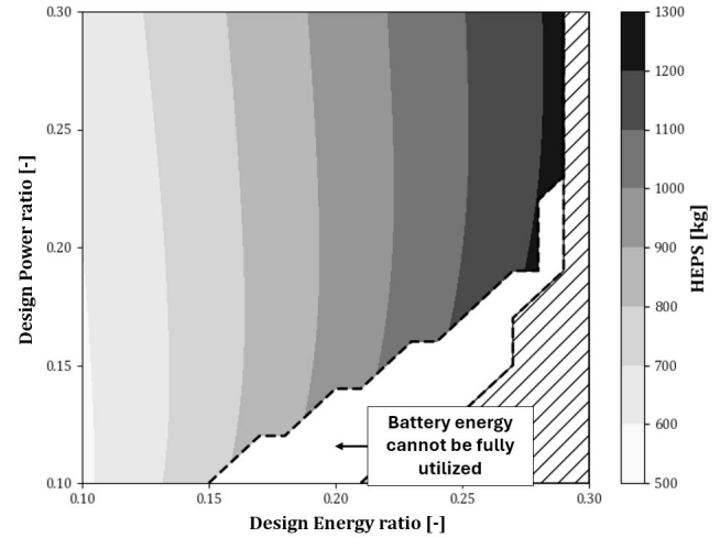
Figure 12. HEPS weight - Double-Leg Mission; PMS optimization
