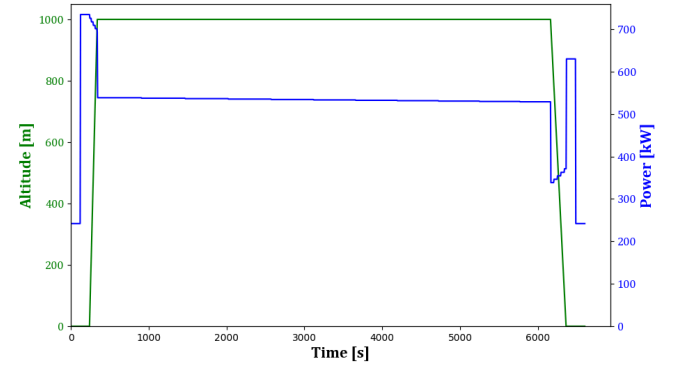
Figure 8. Altitude and power profile - Single-Leg mission
