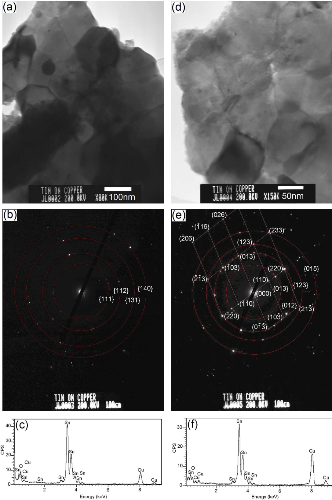
Fig. 8 TEM results of particles removed from the surface of coating AC1: (a) TEM image of one Sn particle; (b) selected area ED spots distributed along the diffraction rings drawn for \text{SnO}_2 ; (c) EDXS spectrum showing relatively higher O content around the selected area; (d) TEM image of another Sn particle; (e) selected area ED spots of zone [3\bar{3}1] or distributed along the diffraction rings drawn for Sn; and (f) EDXS spectrum showing low O content around this selected area.
