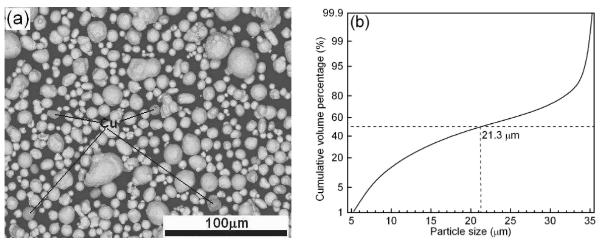
Fig. 1 (a) SEM image and (b) cumulative particle size of the mechanically blended 95wt% Sn plus 5wt% Cu powder feedstock.
