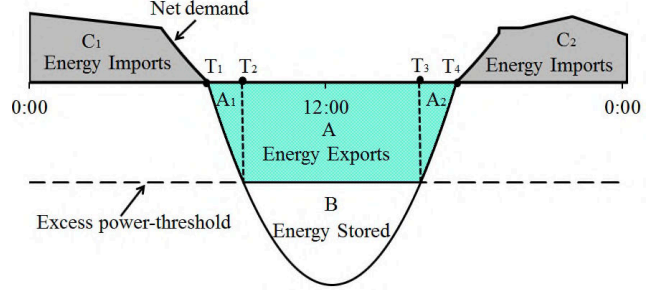
Fig. 3. A residential net demand profile with PV.
